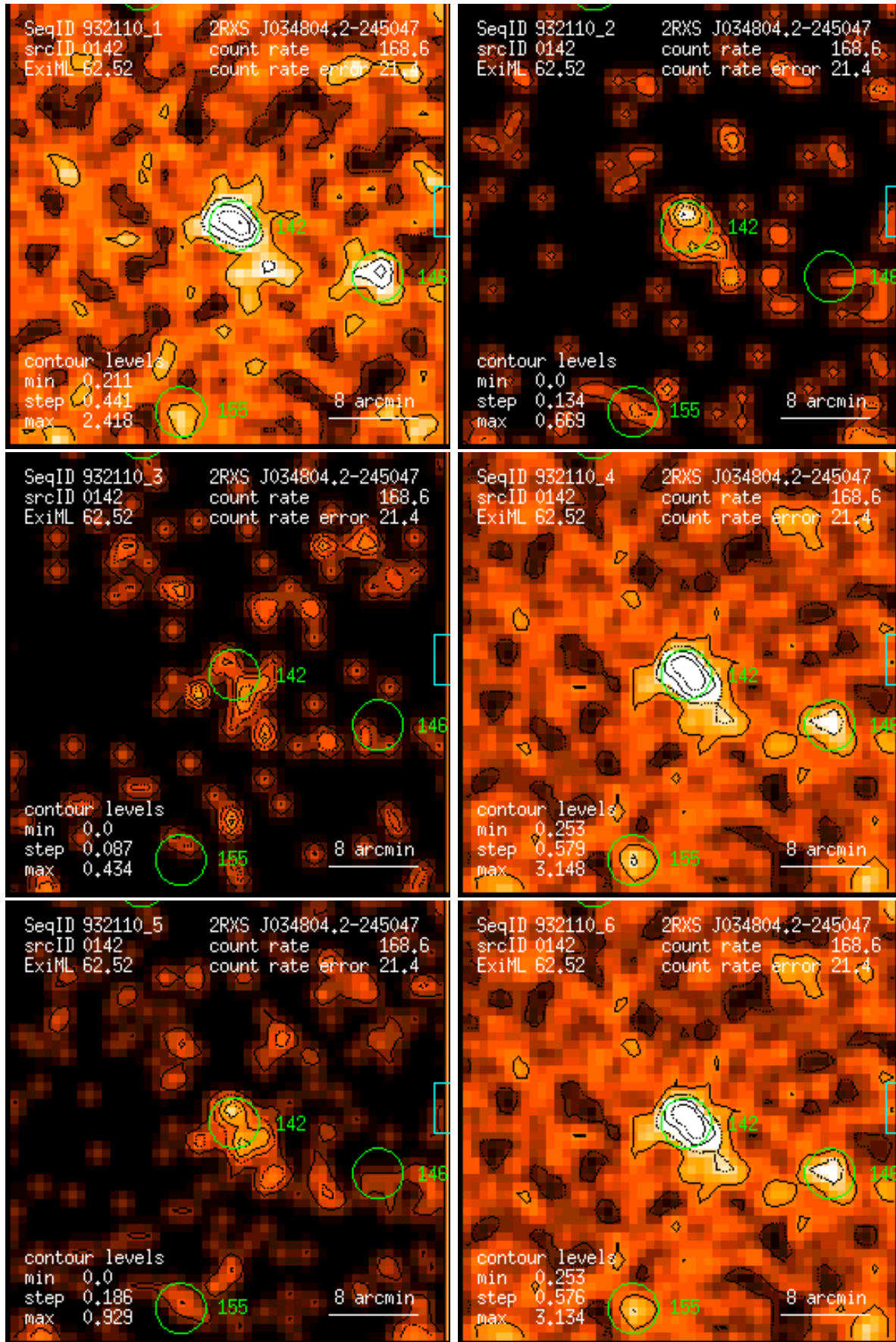
Figure 142: RASS 932110: detection 0142: band rate images, Gaussian filter: (1) PSPC channels 11 – 41, (2) 52 – 90, (3) 91 – 201, (4) 11 – 235, (5) 52 – 201, (6) 11 – 201. Broad band rates in counts/ks. Band rate contour levels in counts/ks/arcmin 2 .
