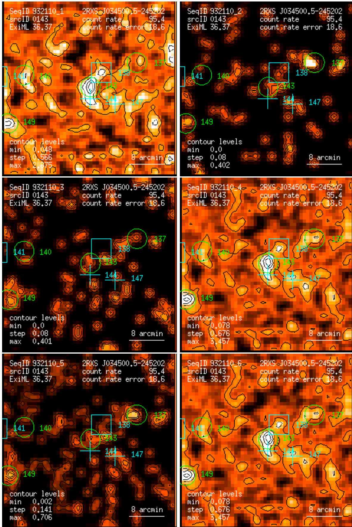
Figure 143: RASS 932110: detection 0143: band rate images, Gaussian filter: (1) PSPC channels 11 – 41, (2) 52 – 90, (3) 91 – 201, (4) 11 – 235, (5) 52 – 201, (6) 11 – 201. Broad band rates in counts/ks. Band rate contour levels in counts/ks/arcmin 2 .
