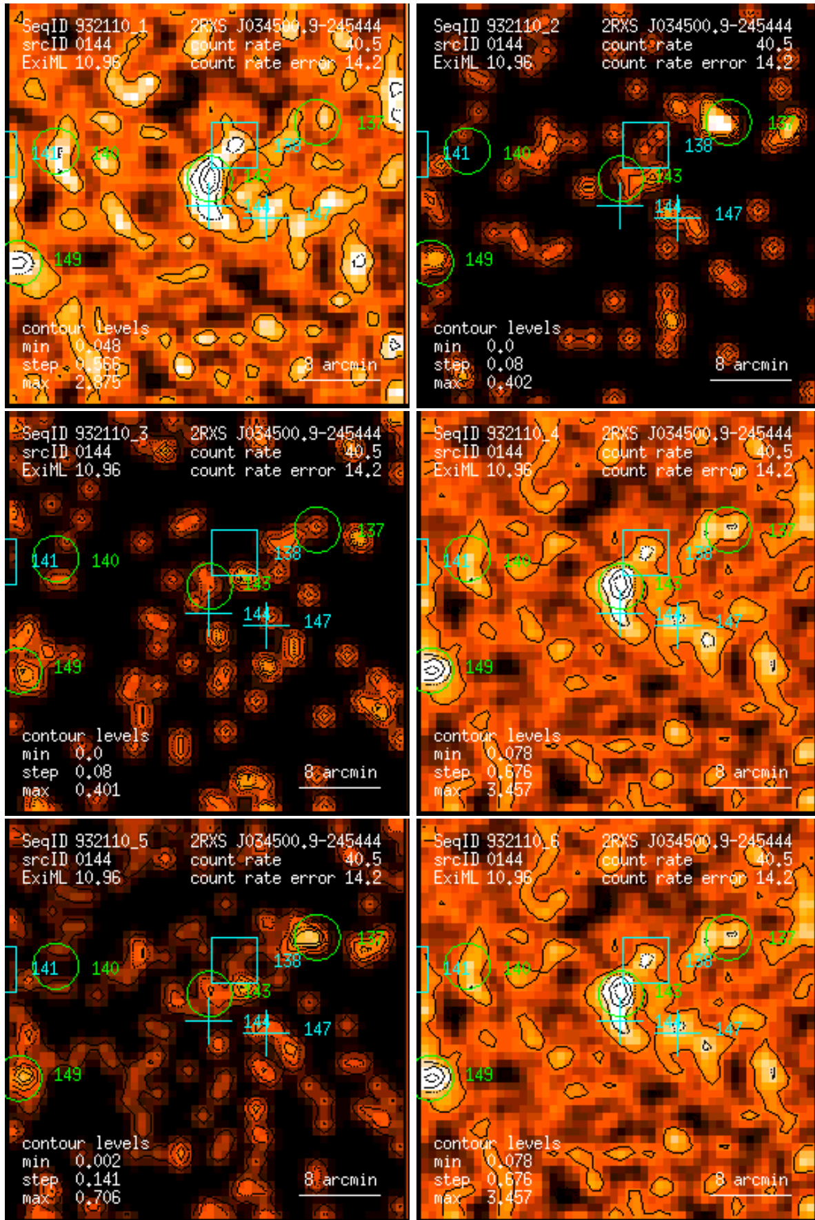
Figure 144: RASS 932110: detection 0144: band rate images, Gaussian filter: (1) PSPC channels 11 – 41, (2) 52 – 90, (3) 91 – 201, (4) 11 – 235, (5) 52 – 201, (6) 11 – 201. Broad band rates in counts/ks. Band rate contour levels in counts/ks/arcmin 2 .
