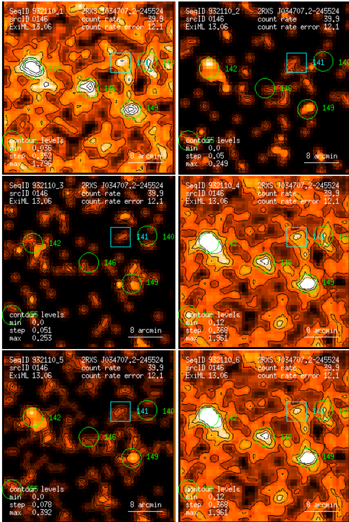
Figure 146: RASS 932110: detection 0146: band rate images, Gaussian filter: (1) PSPC channels 11 – 41, (2) 52 – 90, (3) 91 – 201, (4) 11 – 235, (5) 52 – 201, (6) 11 – 201. Broad band rates in counts/ks. Band rate contour levels in counts/ks/arcmin 2 .
