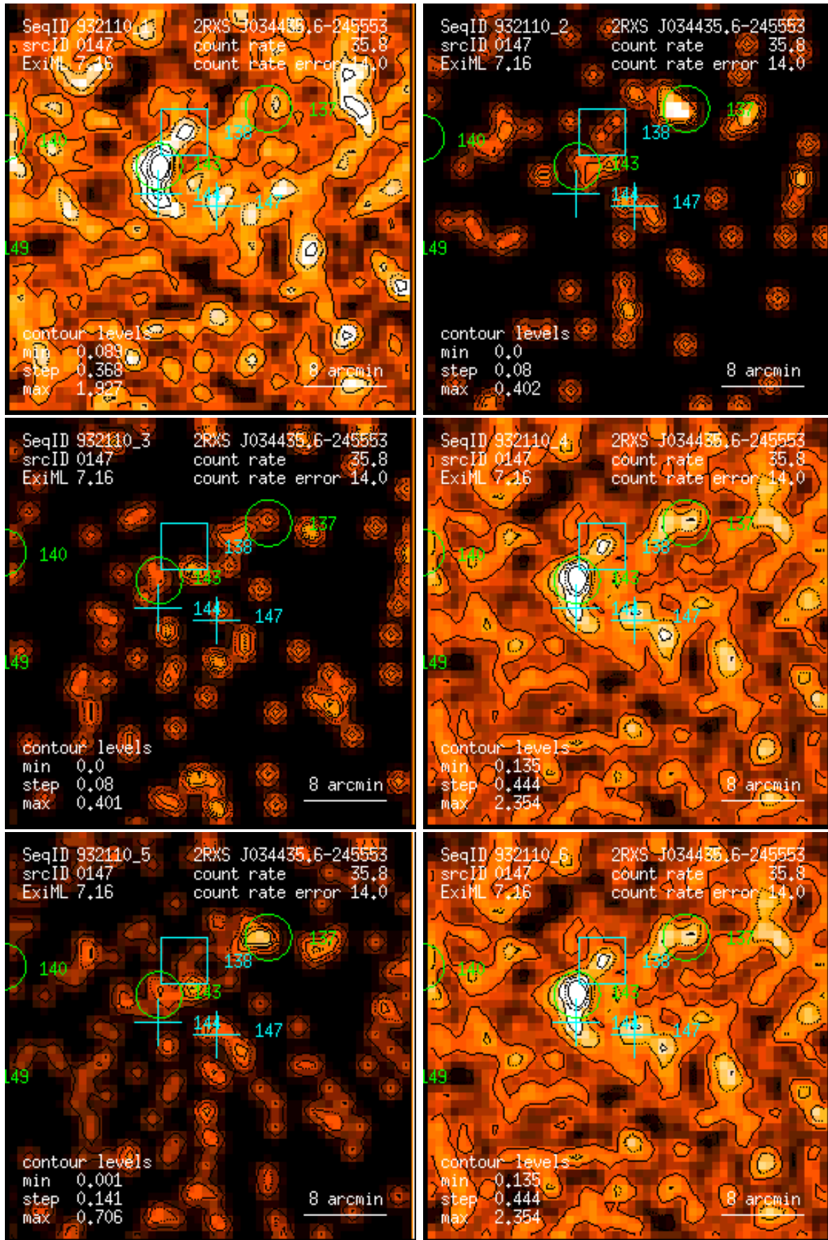
Figure 147: RASS 932110: detection 0147: band rate images, Gaussian filter: (1) PSPC channels 11 – 41, (2) 52 – 90, (3) 91 – 201, (4) 11 – 235, (5) 52 – 201, (6) 11 – 201. Broad band rates in counts/ks. Band rate contour levels in counts/ks/arcmin 2 .
