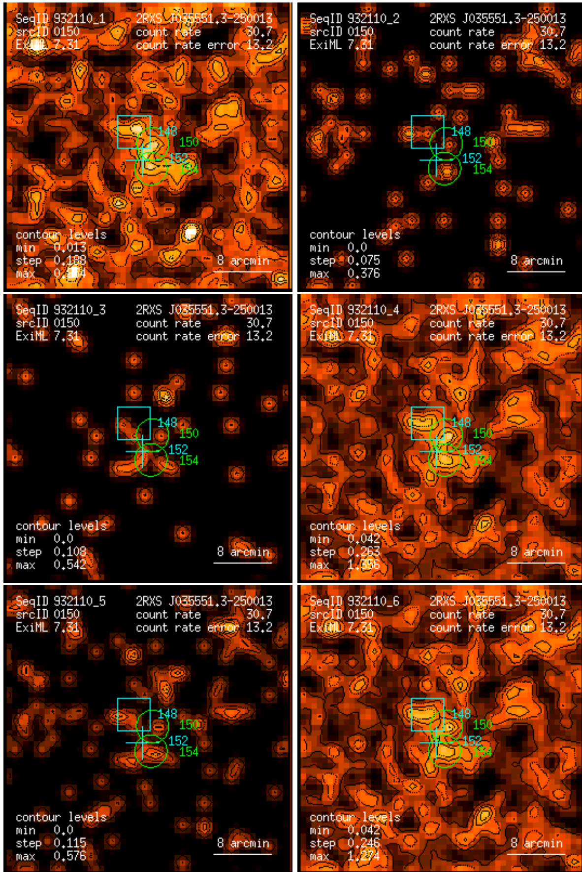
Figure 150: RASS 932110: detection 0150: band rate images, Gaussian filter: (1) PSPC channels 11 – 41, (2) 52 – 90, (3) 91 – 201, (4) 11 – 235, (5) 52 – 201, (6) 11 – 201. Broad band rates in counts/ks. Band rate contour levels in counts/ks/arcmin 2 .
