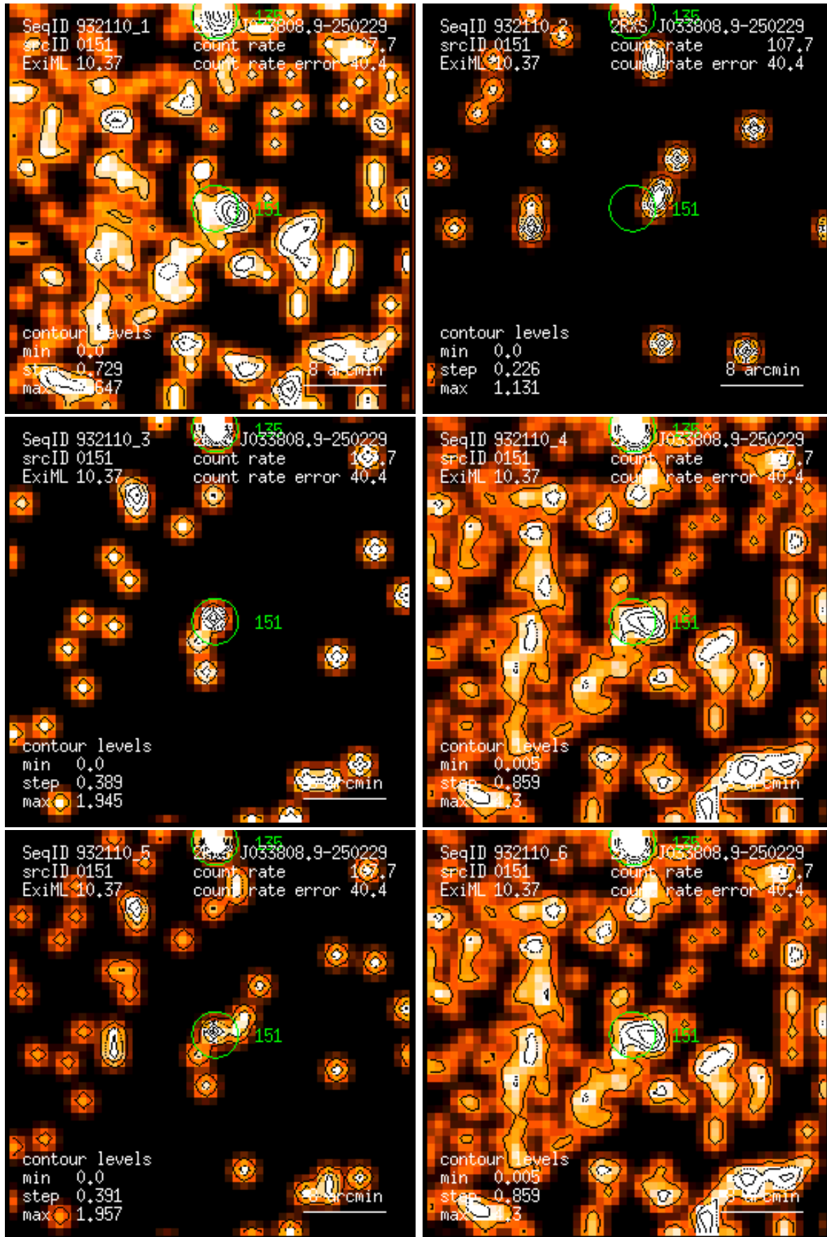
Figure 151: RASS 932110: detection 0151: band rate images, Gaussian filter: (1) PSPC channels 11 – 41, (2) 52 – 90, (3) 91 – 201, (4) 11 – 235, (5) 52 – 201, (6) 11 – 201. Broad band rates in counts/ks. Band rate contour levels in counts/ks/arcmin 2 .
