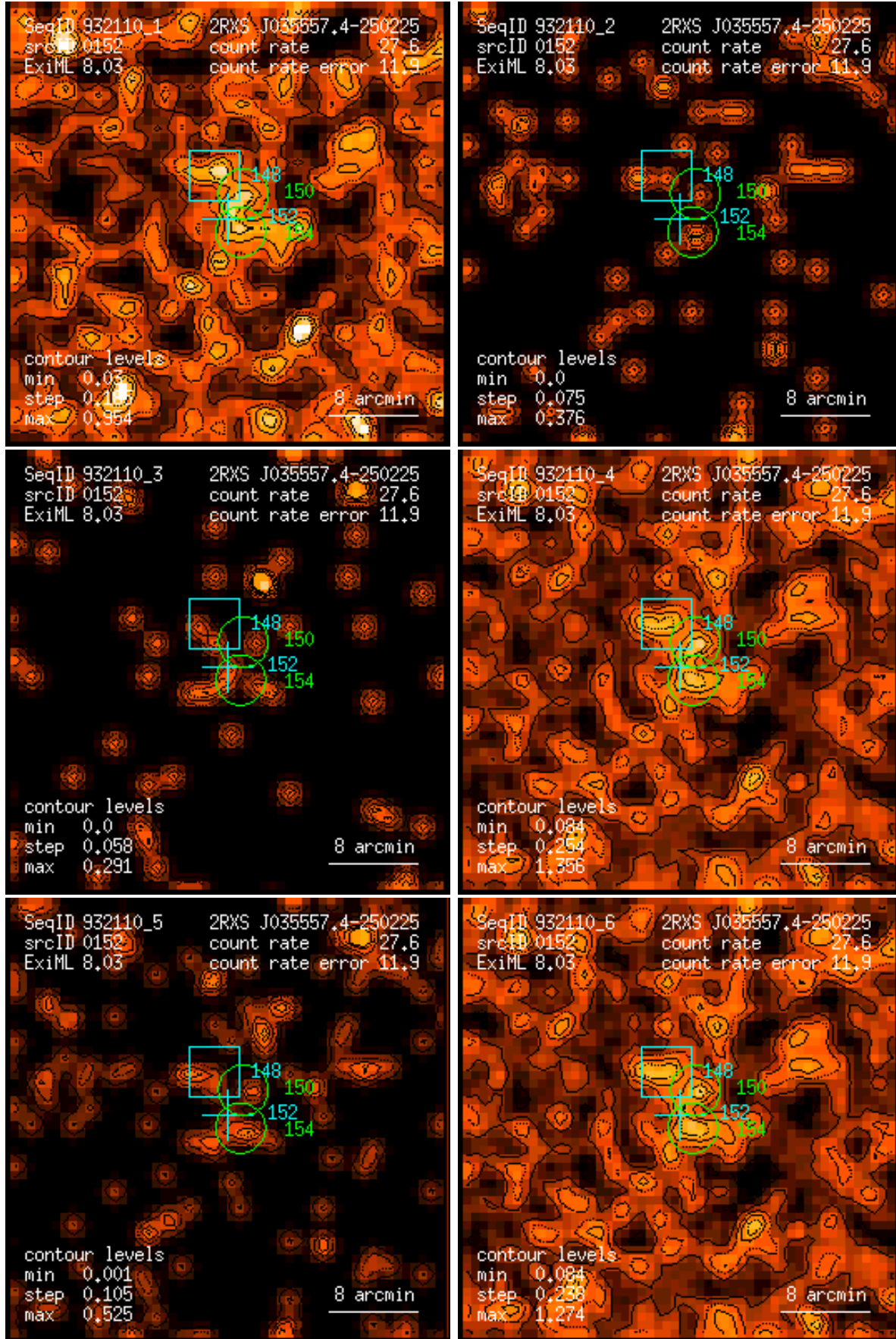
Figure 152: RASS 932110: detection 0152: band rate images, Gaussian filter: (1) PSPC channels 11 – 41, (2) 52 – 90, (3) 91 – 201, (4) 11 – 235, (5) 52 – 201, (6) 11 – 201. Broad band rates in counts/ks. Band rate contour levels in counts/ks/arcmin 2 .
