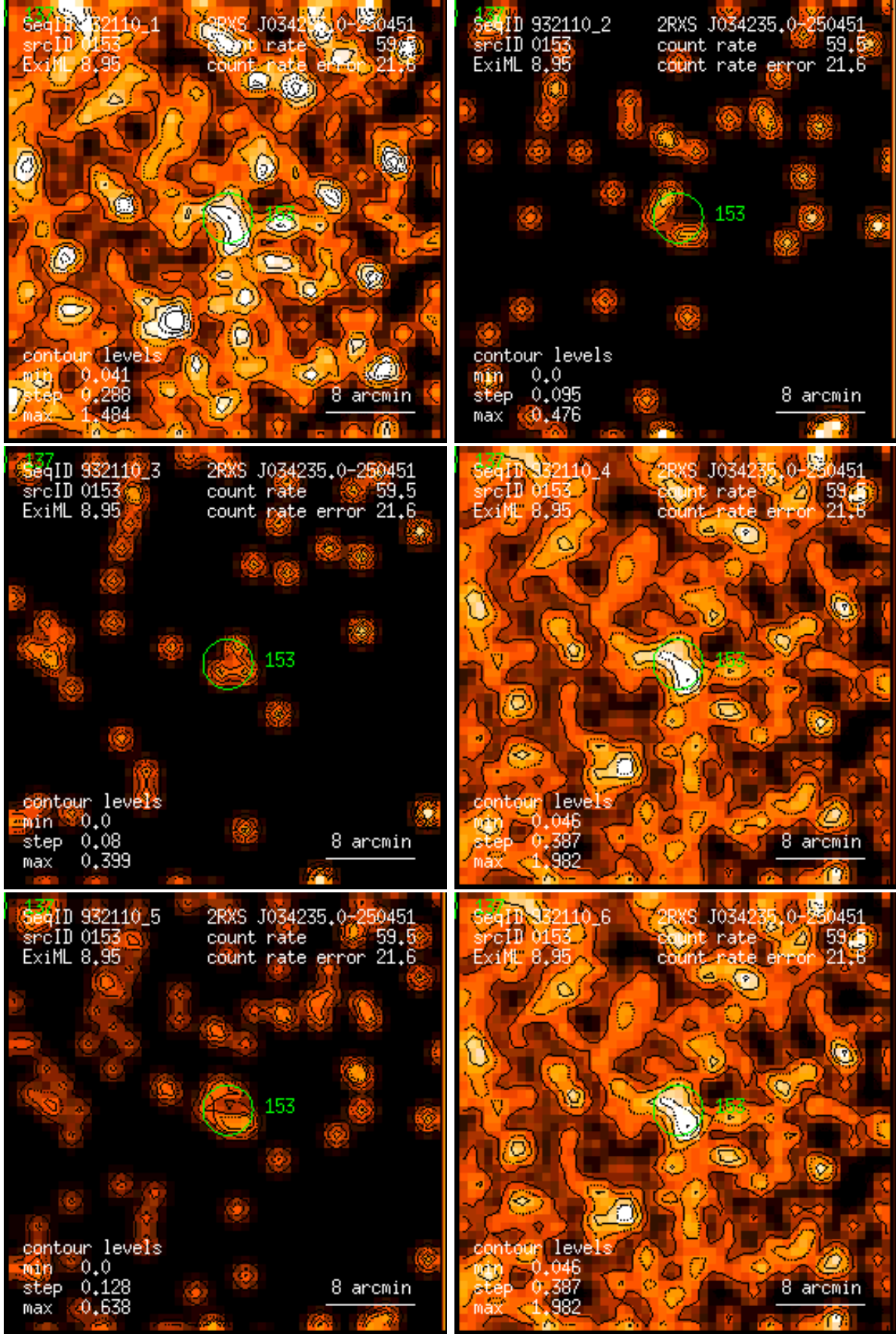
Figure 153: RASS 932110: detection 0153: band rate images, Gaussian filter: (1) PSPC channels 11 – 41, (2) 52 – 90, (3) 91 – 201, (4) 11 – 235, (5) 52 – 201, (6) 11 – 201. Broad band rates in counts/ks. Band rate contour levels in counts/ks/arcmin 2 .
