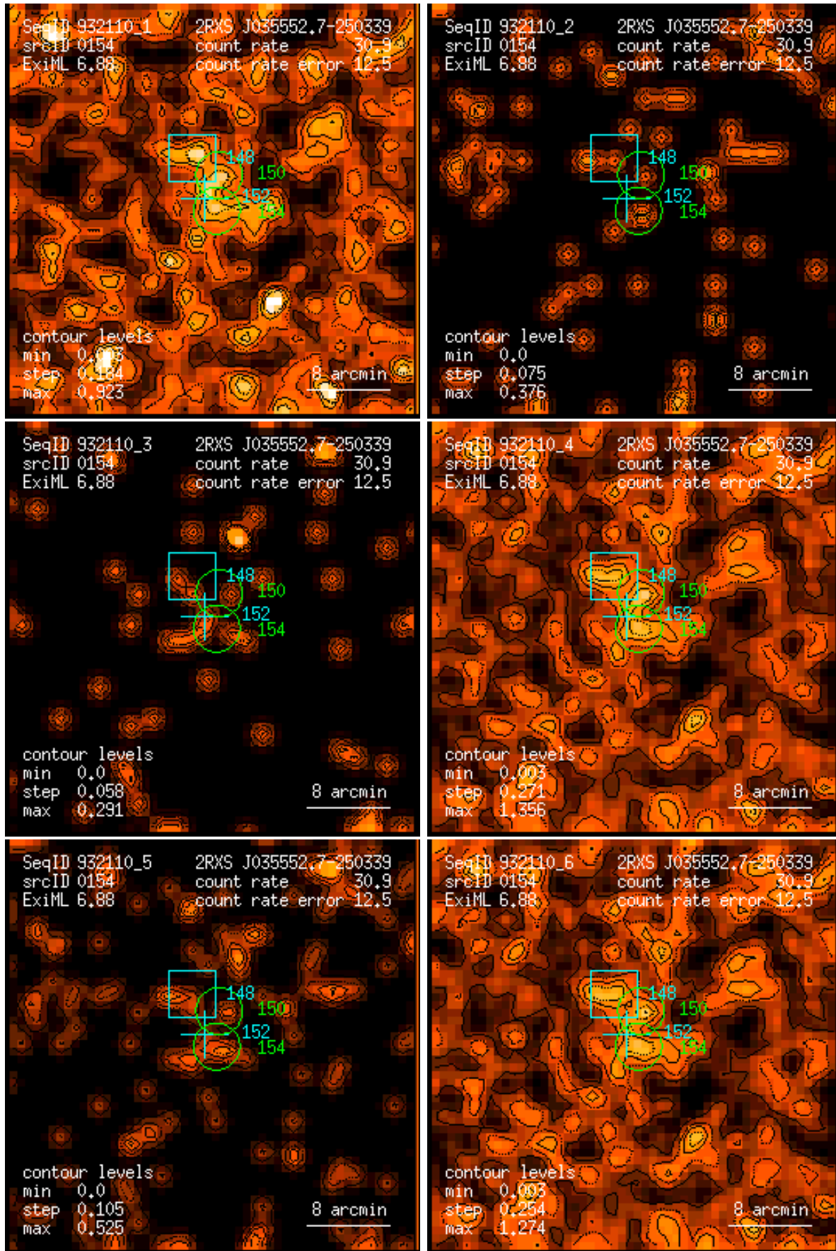
Figure 154: RASS 932110: detection 0154: band rate images, Gaussian filter: (1) PSPC channels 11 – 41, (2) 52 – 90, (3) 91 – 201, (4) 11 – 235, (5) 52 – 201, (6) 11 – 201. Broad band rates in counts/ks. Band rate contour levels in counts/ks/arcmin 2 .
