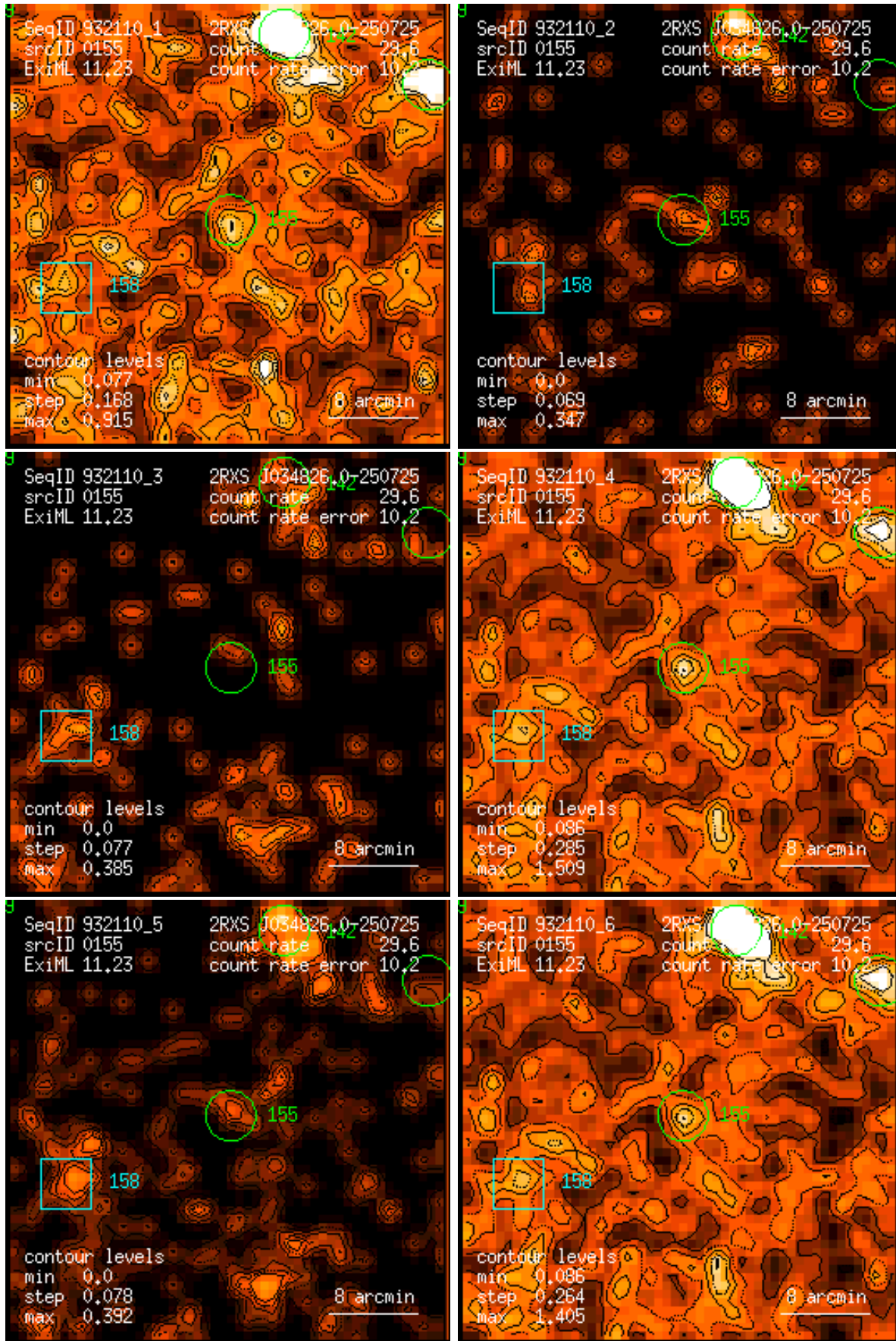
Figure 155: RASS 932110: detection 0155: band rate images, Gaussian filter: (1) PSPC channels 11 – 41, (2) 52 – 90, (3) 91 – 201, (4) 11 – 235, (5) 52 – 201, (6) 11 – 201. Broad band rates in counts/ks. Band rate contour levels in counts/ks/arcmin 2 .
