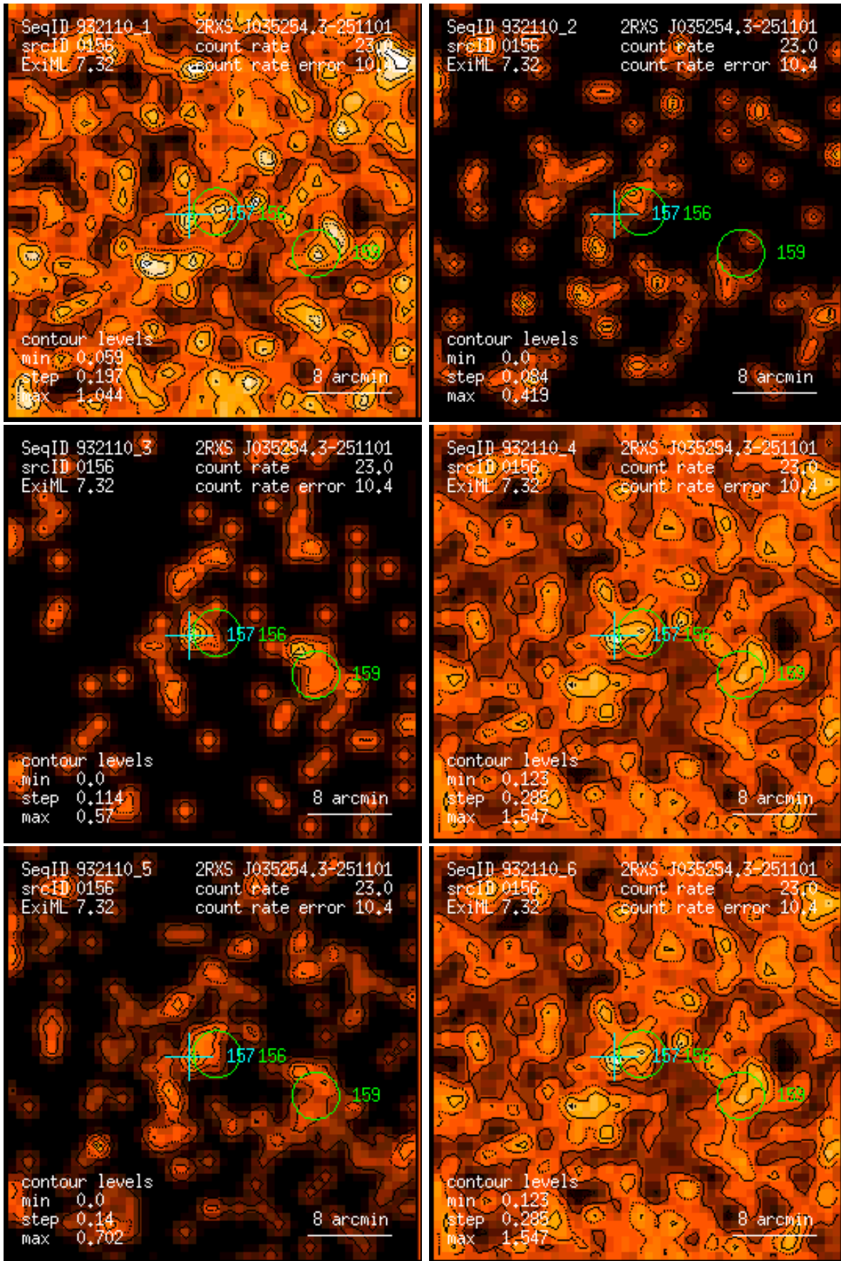
Figure 156: RASS 932110: detection 0156: band rate images, Gaussian filter: (1) PSPC channels 11 – 41, (2) 52 – 90, (3) 91 – 201, (4) 11 – 235, (5) 52 – 201, (6) 11 – 201. Broad band rates in counts/ks. Band rate contour levels in counts/ks/arcmin 2 .
