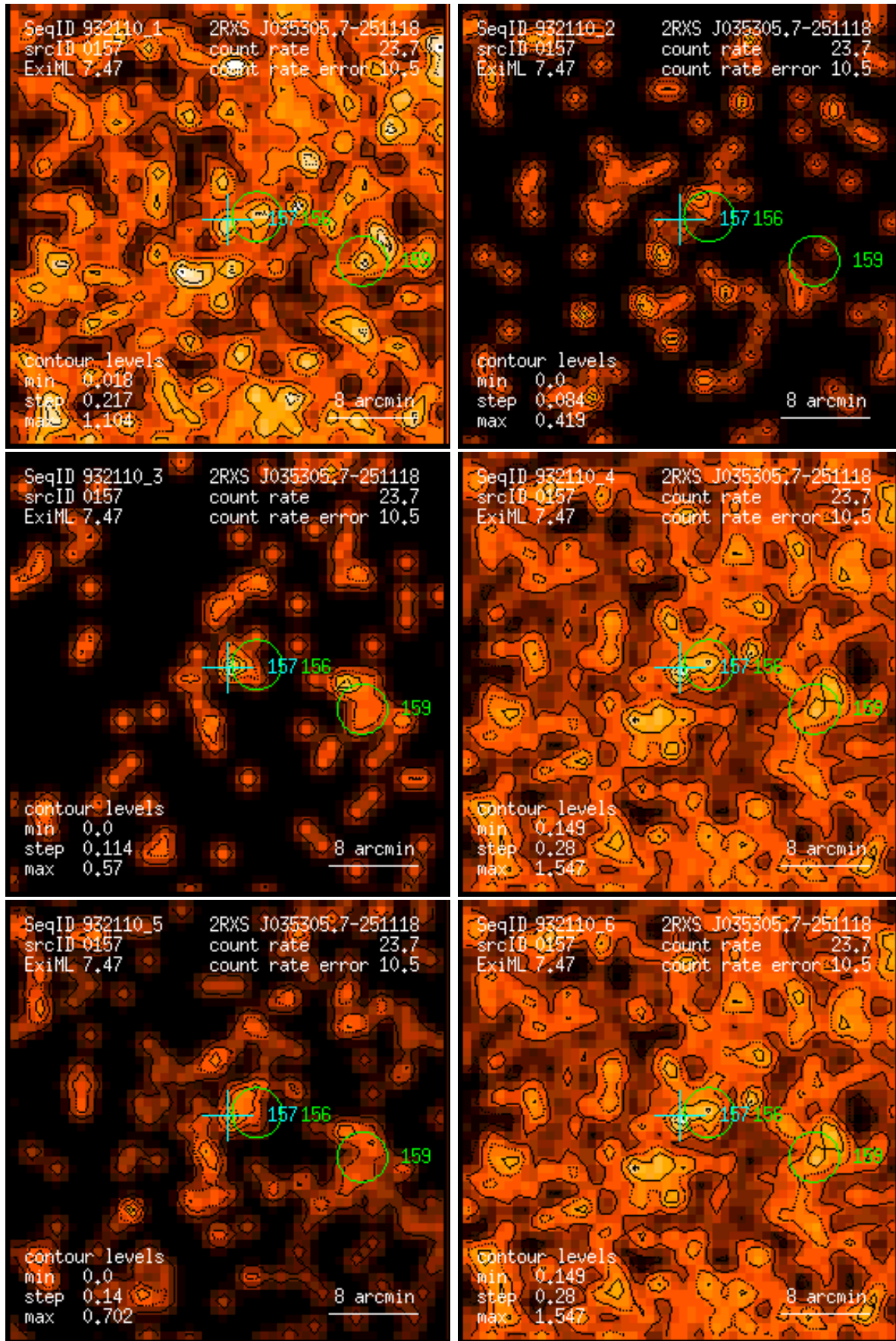
Figure 157: RASS 932110: detection 0157: band rate images, Gaussian filter: (1) PSPC channels 11 – 41, (2) 52 – 90, (3) 91 – 201, (4) 11 – 235, (5) 52 – 201, (6) 11 – 201. Broad band rates in counts/ks. Band rate contour levels in counts/ks/arcmin 2 .
