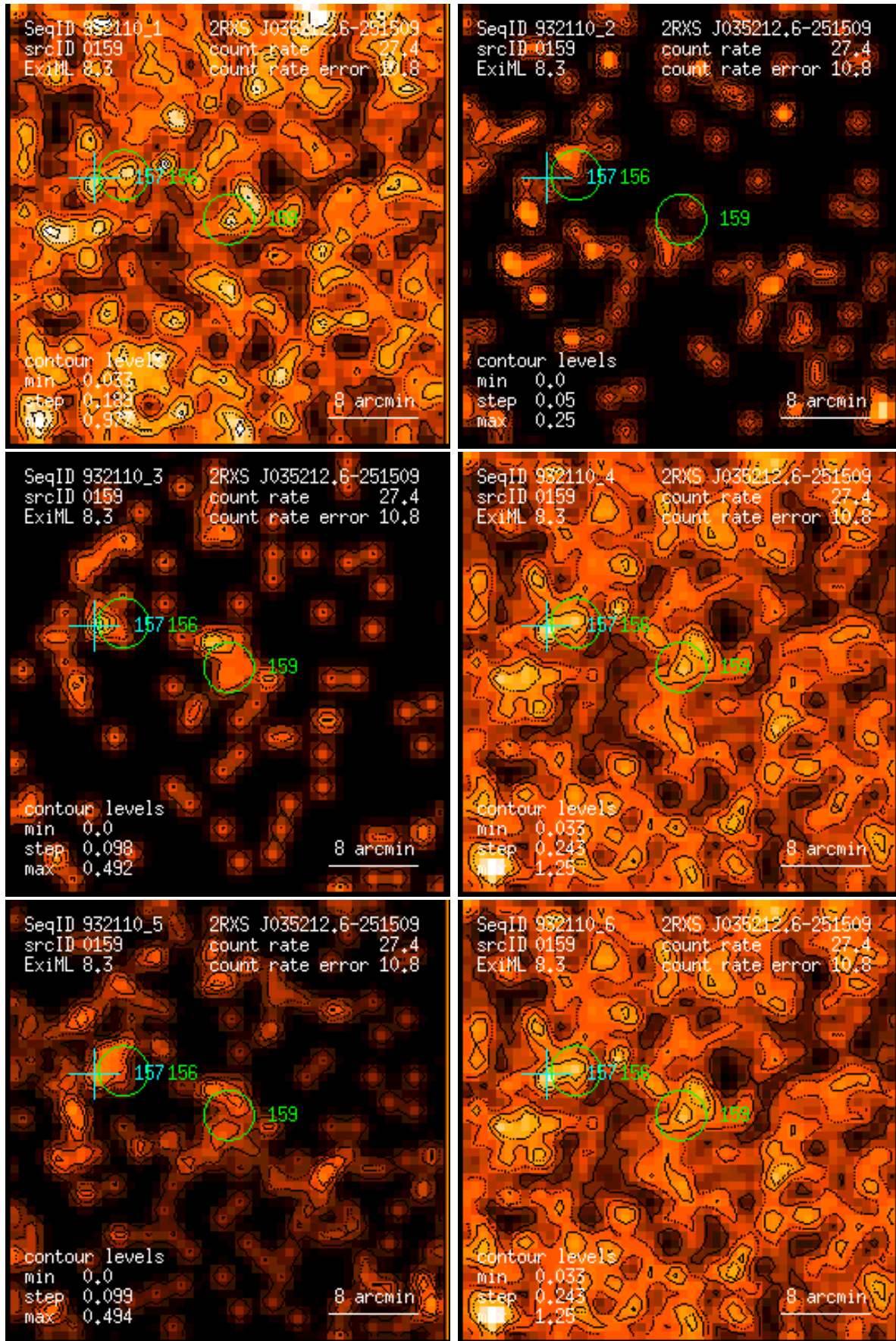
Figure 159: RASS 932110: detection 0159: band rate images, Gaussian filter: (1) PSPC channels 11 – 41, (2) 52 – 90, (3) 91 – 201, (4) 11 – 235, (5) 52 – 201, (6) 11 – 201. Broad band rates in counts/ks. Band rate contour levels in counts/ks/arcmin 2 .
