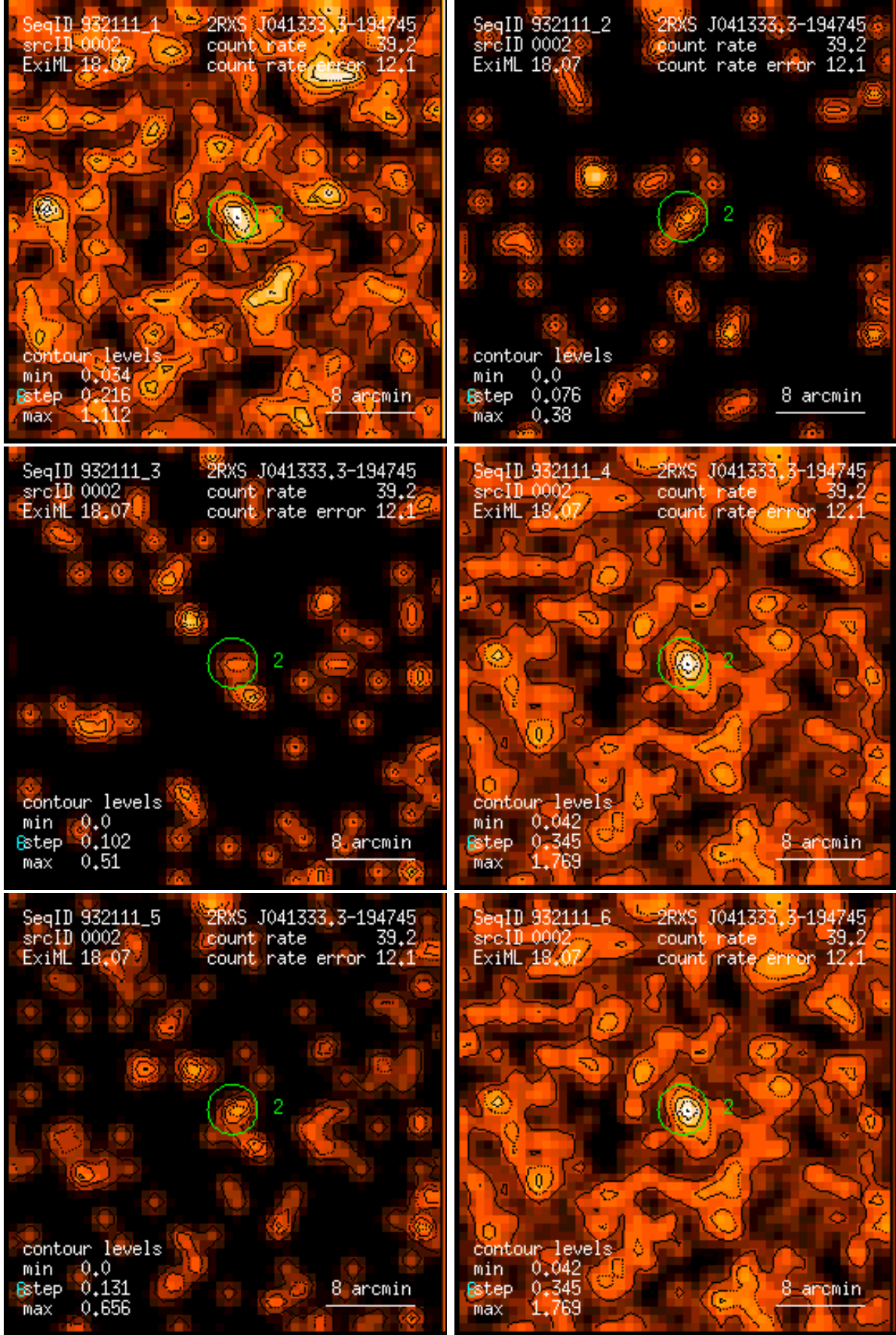
Figure 2: RASS 932111: detection 0002: band rate images, Gaussian filter: (1) PSPC channels 11 – 41, (2) 52 – 90, (3) 91 – 201, (4) 11 – 235, (5) 52 – 201, (6) 11 – 201. Broad band rates in counts/ks. Band rate contour levels in counts/ks/arcmin 2 .
