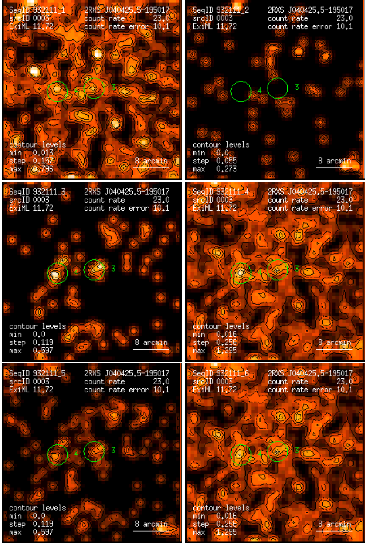
Figure 3: RASS 932111: detection 0003: band rate images, Gaussian filter: (1) PSPC channels 11 – 41, (2) 52 – 90, (3) 91 – 201, (4) 11 – 235, (5) 52 – 201, (6) 11 – 201. Broad band rates in counts/ks. Band rate contour levels in counts/ks/arcmin 2 .
