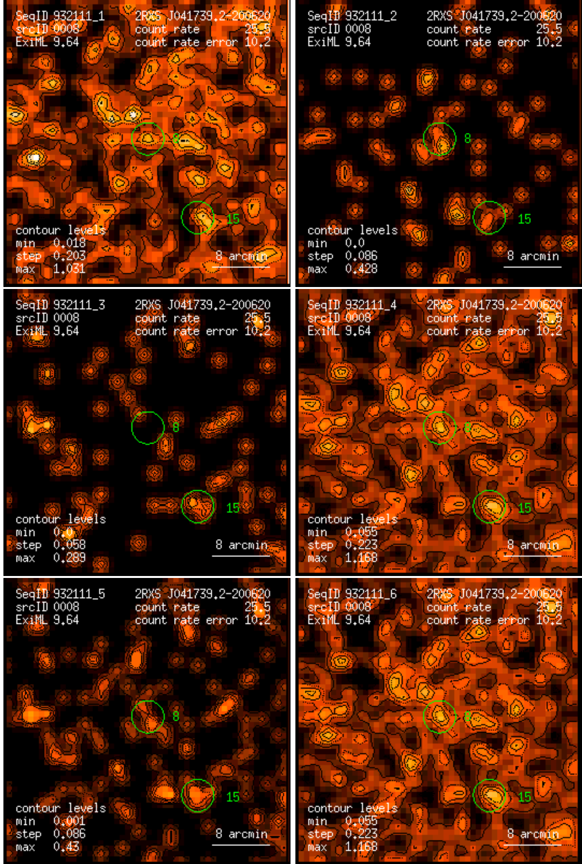
Figure 8: RASS 932111: detection 0008: band rate images, Gaussian filter: (1) PSPC channels 11 – 41, (2) 52 – 90, (3) 91 – 201, (4) 11 – 235, (5) 52 – 201, (6) 11 – 201. Broad band rates in counts/ks. Band rate contour levels in counts/ks/arcmin 2 .
