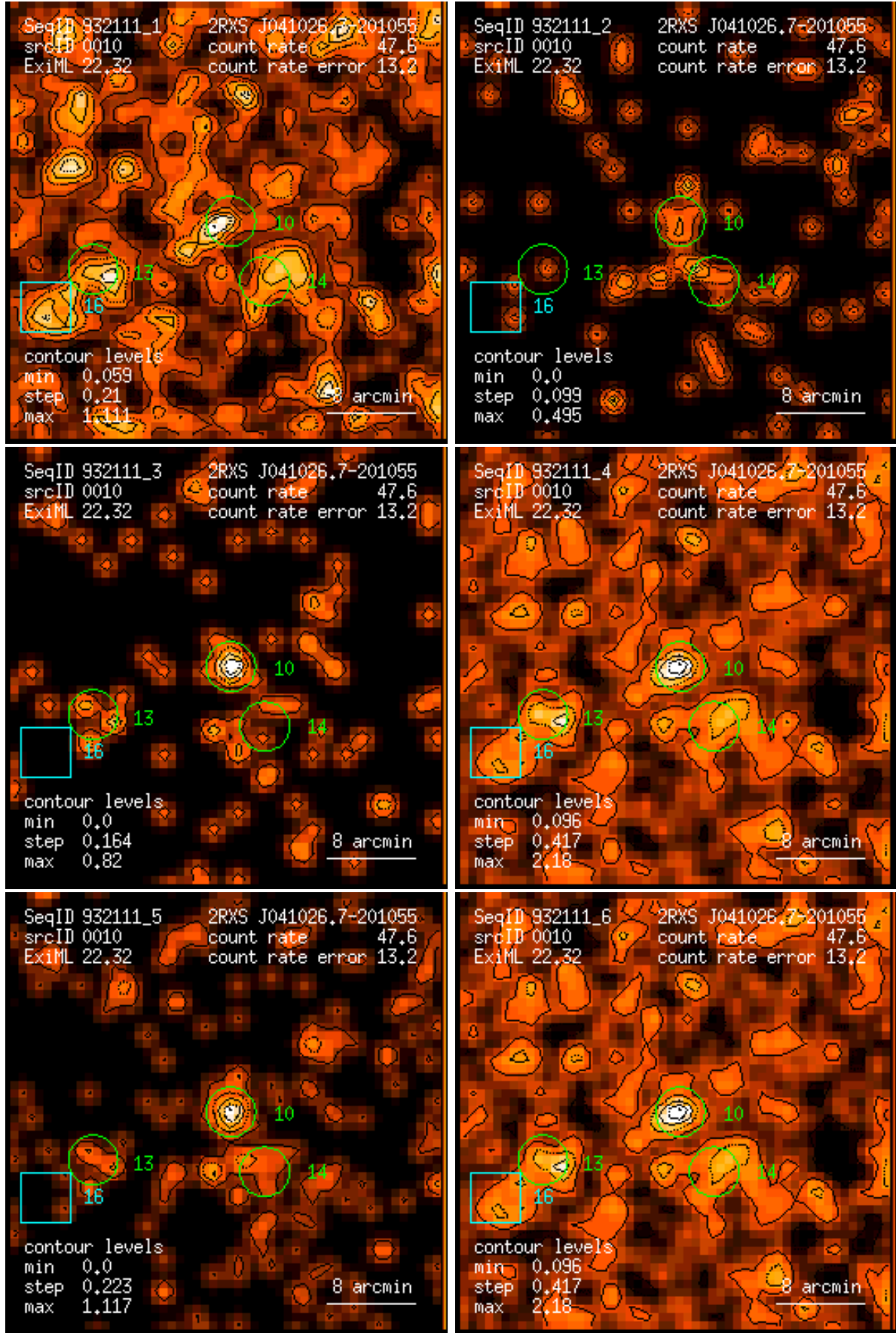
Figure 10: RASS 932111: detection 0010: band rate images, Gaussian filter: (1) PSPC channels 11 – 41, (2) 52 – 90, (3) 91 – 201, (4) 11 – 235, (5) 52 – 201, (6) 11 – 201. Broad band rates in counts/ks. Band rate contour levels in counts/ks/arcmin 2 .
