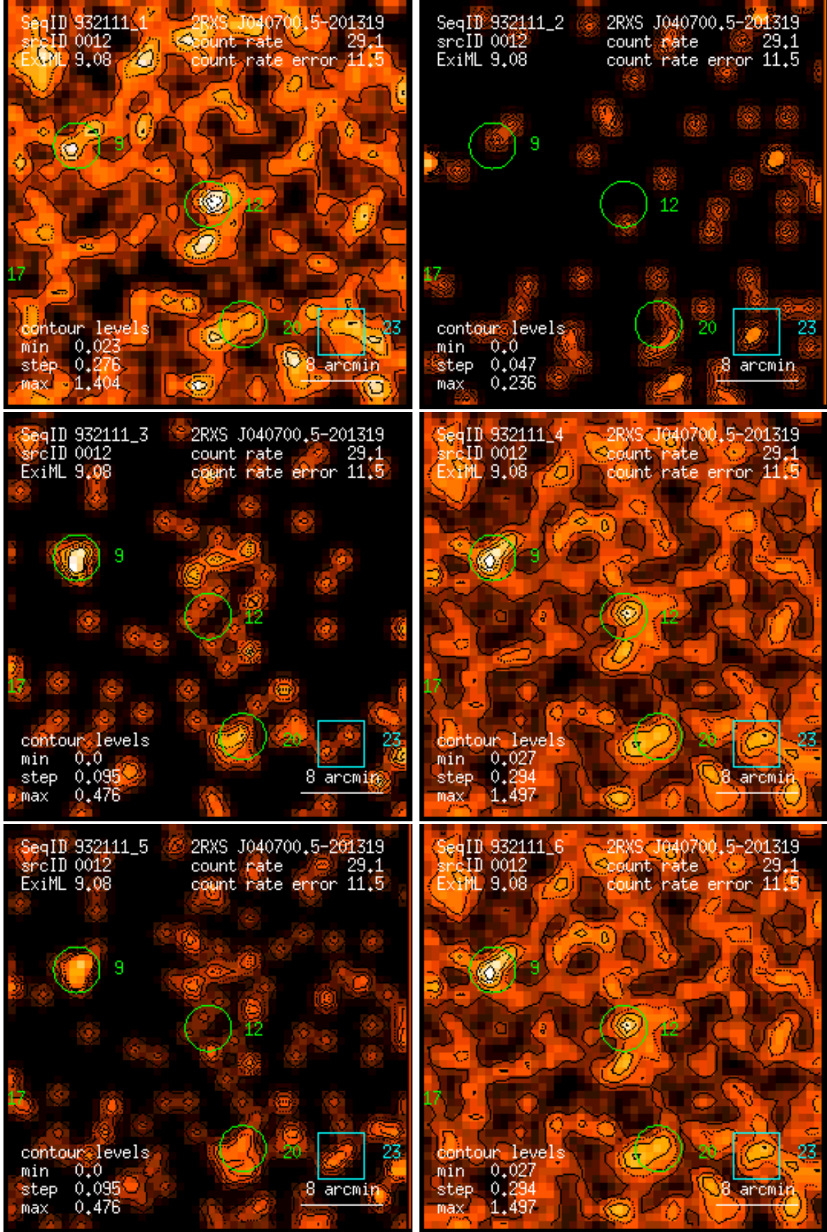
Figure 12: RASS 932111: detection 0012: band rate images, Gaussian filter: (1) PSPC channels 11 – 41, (2) 52 – 90, (3) 91 – 201, (4) 11 – 235, (5) 52 – 201, (6) 11 – 201. Broad band rates in counts/ks. Band rate contour levels in counts/ks/arcmin 2 .
