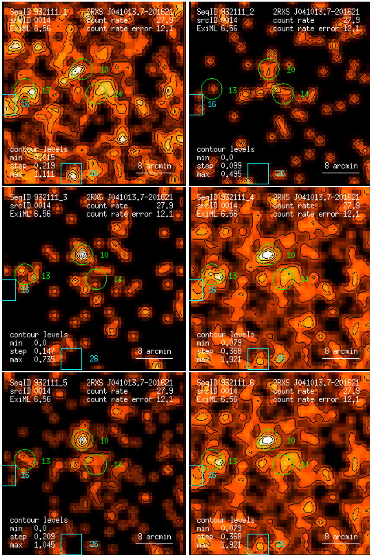
Figure 14: RASS 932111: detection 0014: band rate images, Gaussian filter: (1) PSPC channels 11 – 41, (2) 52 – 90, (3) 91 – 201, (4) 11 – 235, (5) 52 – 201, (6) 11 – 201. Broad band rates in counts/ks. Band rate contour levels in counts/ks/arcmin 2 .
