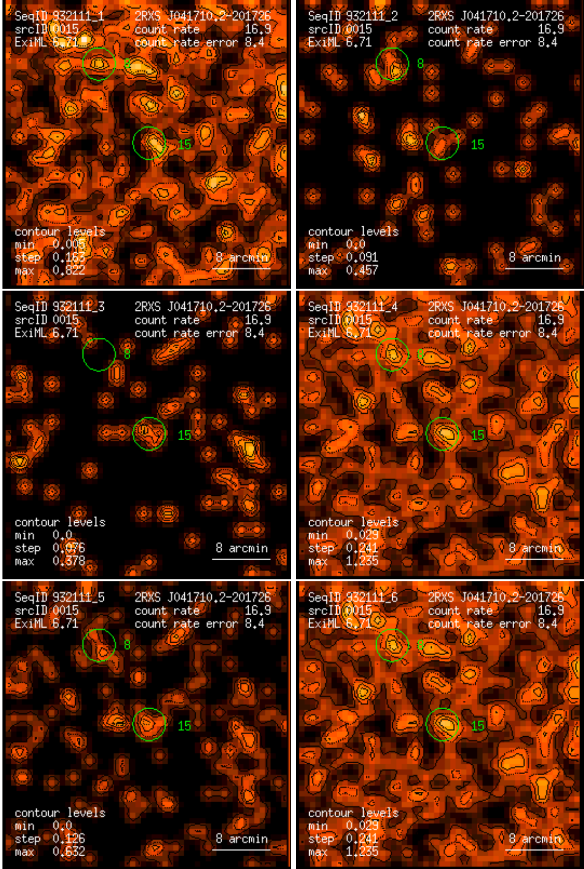
Figure 15: RASS 932111: detection 0015: band rate images, Gaussian filter: (1) PSPC channels 11 – 41, (2) 52 – 90, (3) 91 – 201, (4) 11 – 235, (5) 52 – 201, (6) 11 – 201. Broad band rates in counts/ks. Band rate contour levels in counts/ks/arcmin 2 .
