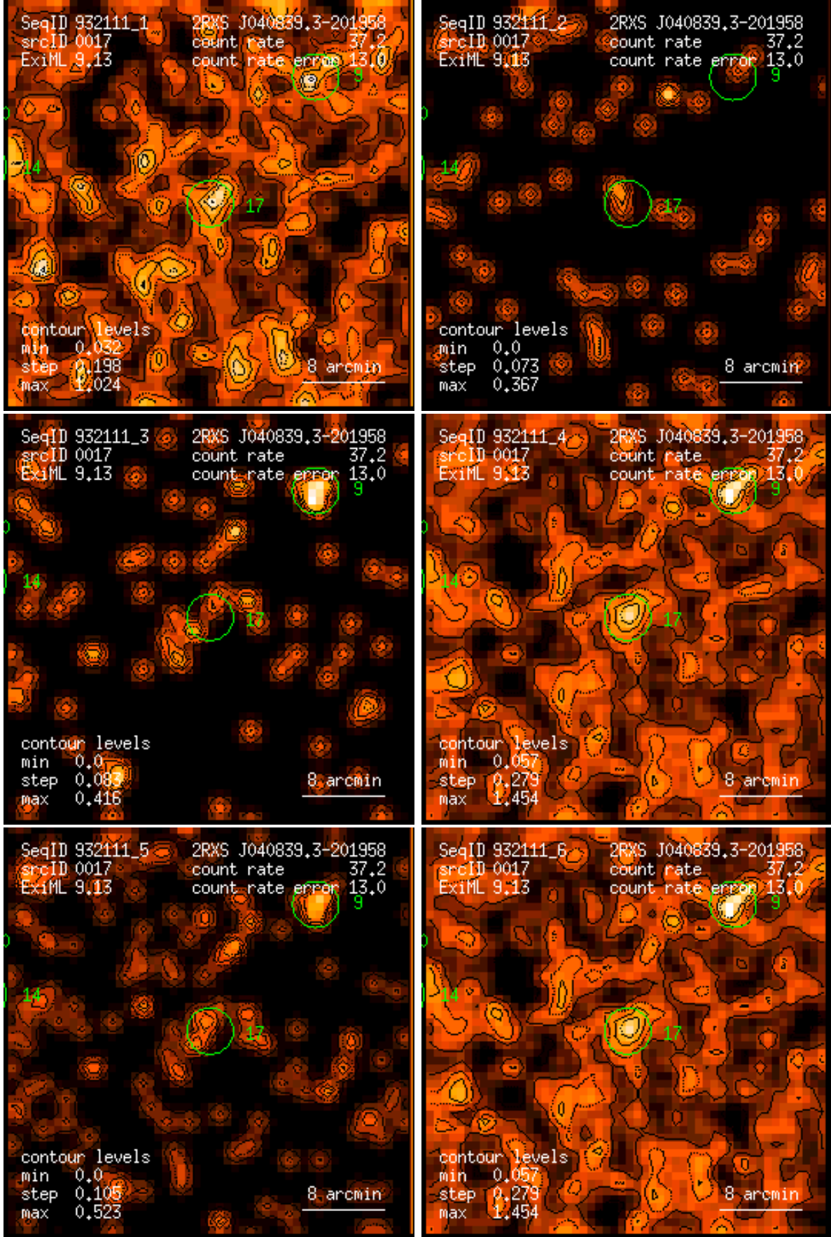
Figure 17: RASS 932111: detection 0017: band rate images, Gaussian filter: (1) PSPC channels 11 – 41, (2) 52 – 90, (3) 91 – 201, (4) 11 – 235, (5) 52 – 201, (6) 11 – 201. Broad band rates in counts/ks. Band rate contour levels in counts/ks/arcmin 2 .
