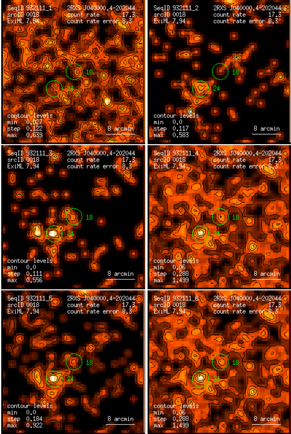
Figure 18: RASS 932111: detection 0018: band rate images, Gaussian filter: (1) PSPC channels 11 – 41, (2) 52 – 90, (3) 91 – 201, (4) 11 – 235, (5) 52 – 201, (6) 11 – 201. Broad band rates in counts/ks. Band rate contour levels in counts/ks/arcmin 2 .
