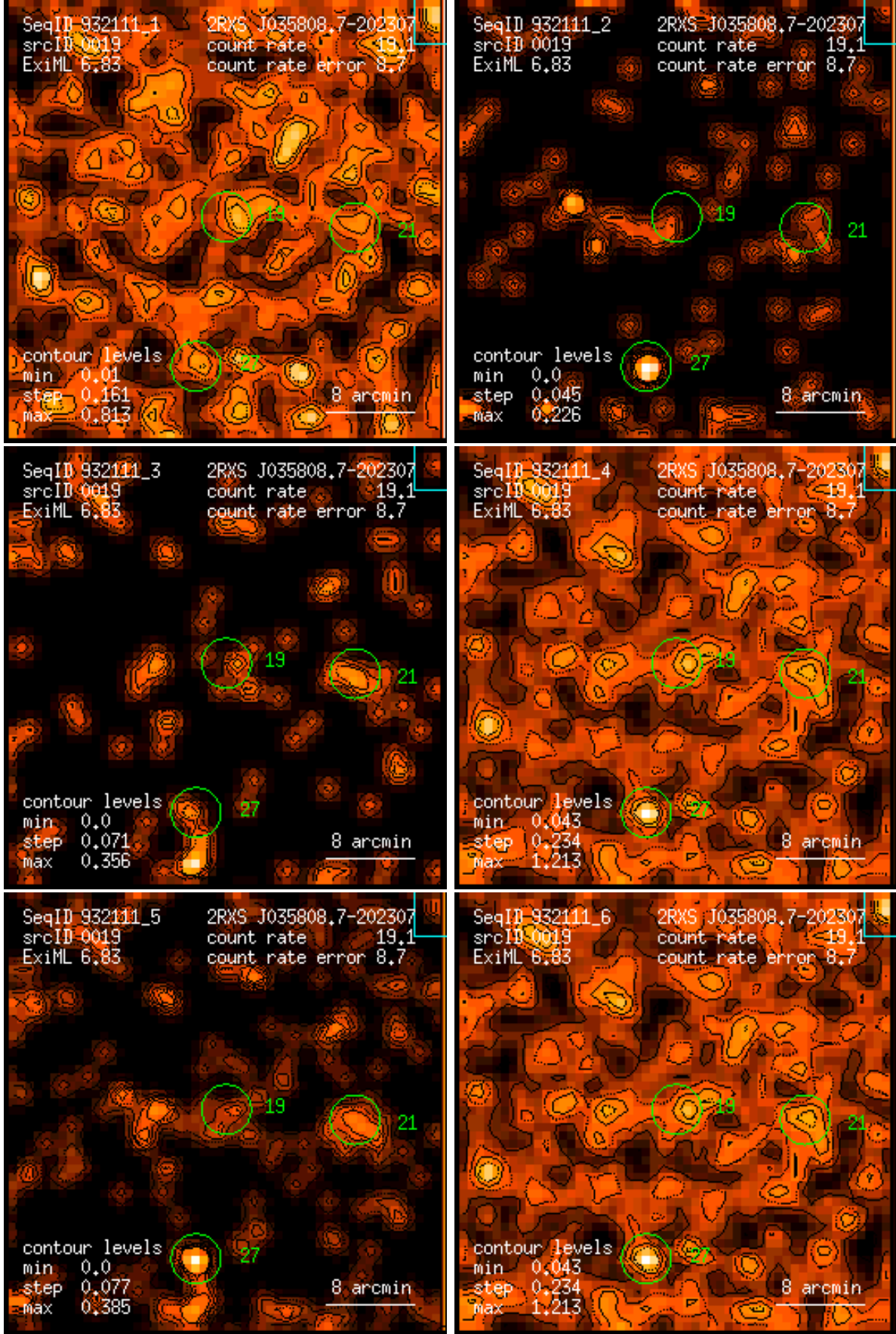
Figure 19: RASS 932111: detection 0019: band rate images, Gaussian filter: (1) PSPC channels 11 – 41, (2) 52 – 90, (3) 91 – 201, (4) 11 – 235, (5) 52 – 201, (6) 11 – 201. Broad band rates in counts/ks. Band rate contour levels in counts/ks/arcmin 2 .
