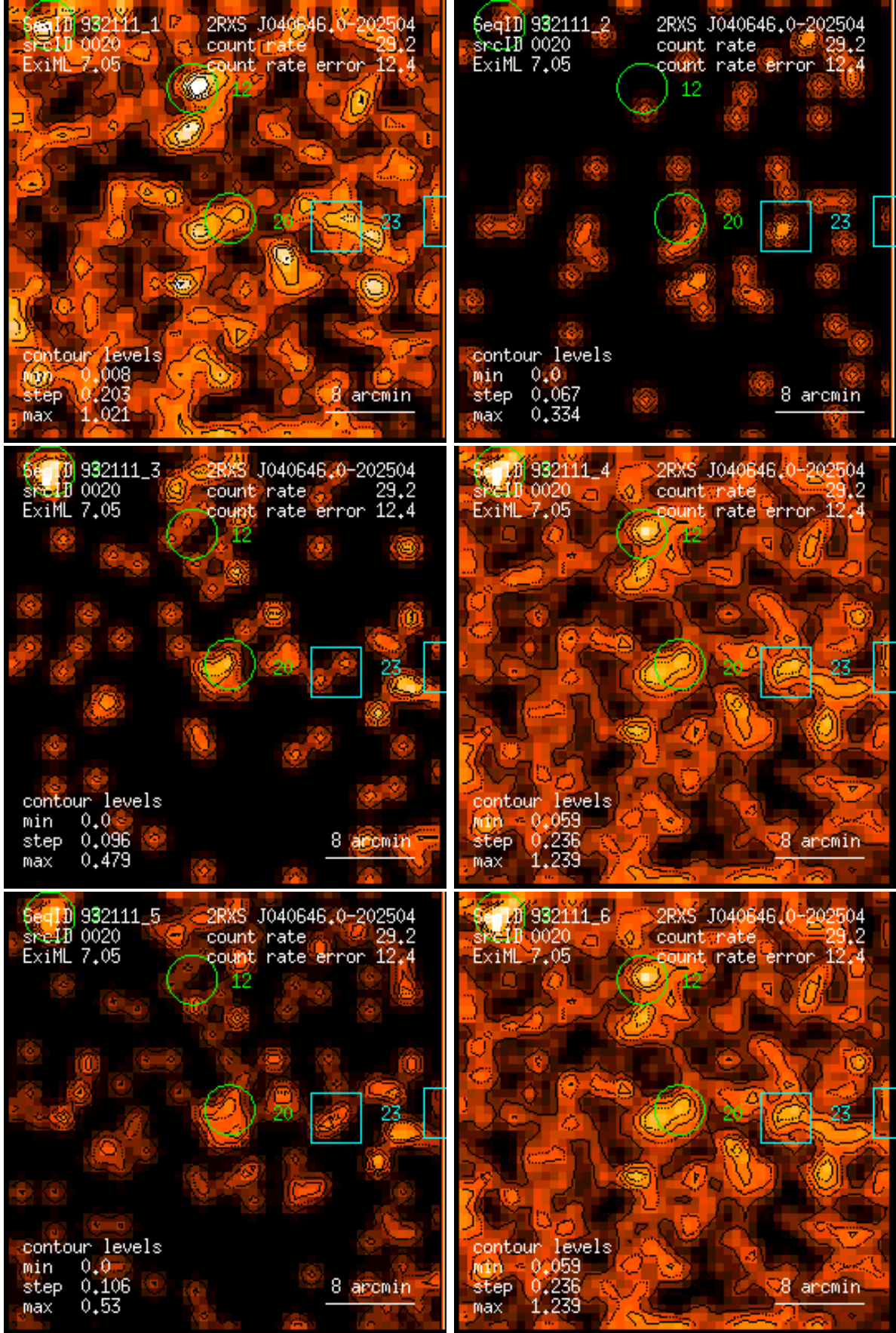
Figure 20: RASS 932111: detection 0020: band rate images, Gaussian filter: (1) PSPC channels 11 – 41, (2) 52 – 90, (3) 91 – 201, (4) 11 – 235, (5) 52 – 201, (6) 11 – 201. Broad band rates in counts/ks. Band rate contour levels in counts/ks/arcmin 2 .
