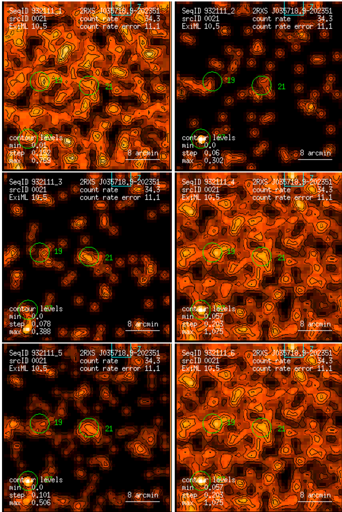
Figure 21: RASS 932111: detection 0021: band rate images, Gaussian filter: (1) PSPC channels 11 – 41, (2) 52 – 90, (3) 91 – 201, (4) 11 – 235, (5) 52 – 201, (6) 11 – 201. Broad band rates in counts/ks. Band rate contour levels in counts/ks/arcmin 2 .
