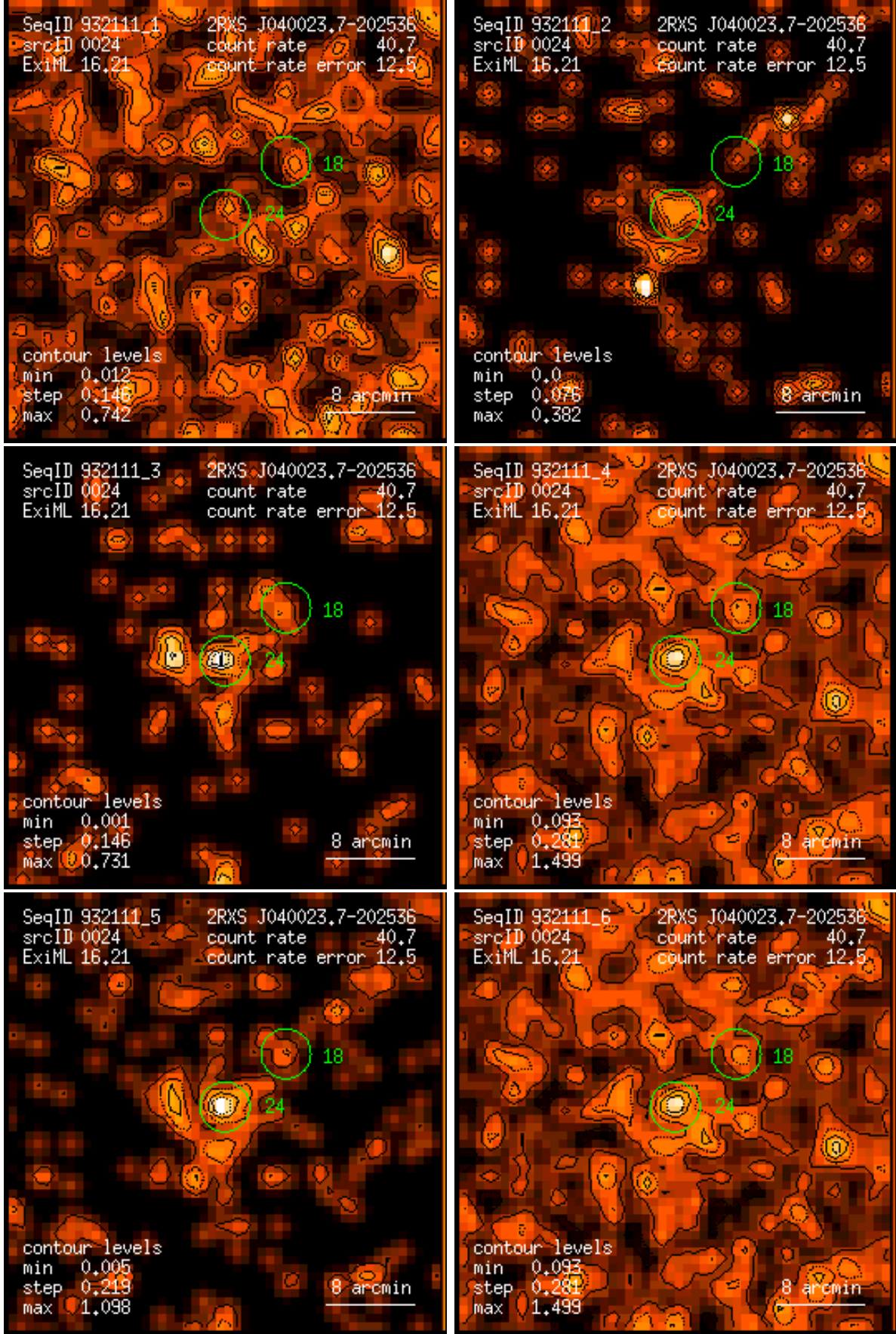
Figure 24: RASS 932111: detection 0024: band rate images, Gaussian filter: (1) PSPC channels 11 – 41, (2) 52 – 90, (3) 91 – 201, (4) 11 – 235, (5) 52 – 201, (6) 11 – 201. Broad band rates in counts/ks. Band rate contour levels in counts/ks/arcmin 2 .
