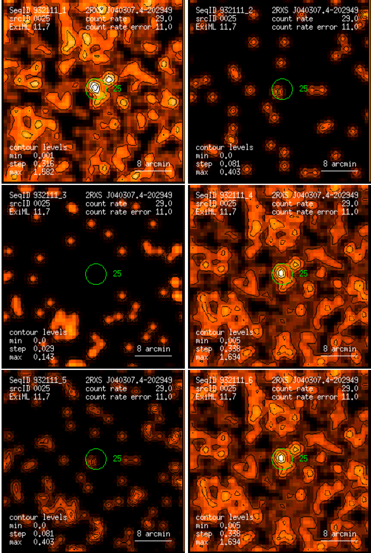
Figure 25: RASS 932111: detection 0025: band rate images, Gaussian filter: (1) PSPC channels 11 – 41, (2) 52 – 90, (3) 91 – 201, (4) 11 – 235, (5) 52 – 201, (6) 11 – 201. Broad band rates in counts/ks. Band rate contour levels in counts/ks/arcmin 2 .
