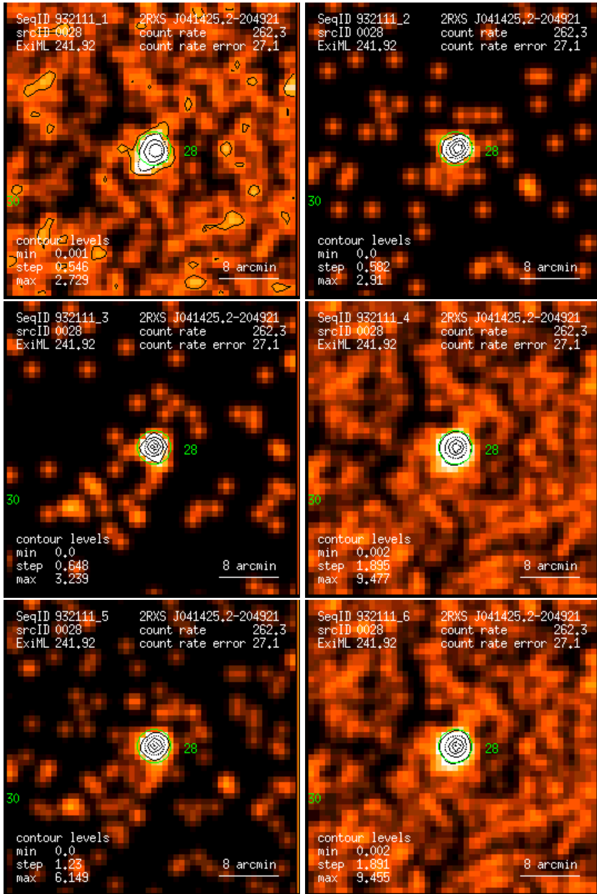
Figure 28: RASS 932111: detection 0028: band rate images, Gaussian filter: (1) PSPC channels 11 – 41, (2) 52 – 90, (3) 91 – 201, (4) 11 – 235, (5) 52 – 201, (6) 11 – 201. Broad band rates in counts/ks. Band rate contour levels in counts/ks/arcmin 2 .
