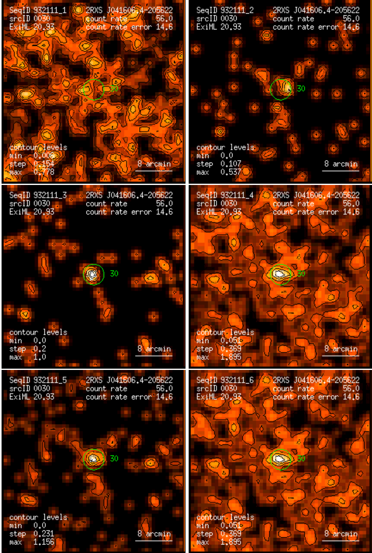
Figure 30: RASS 932111: detection 0030: band rate images, Gaussian filter: (1) PSPC channels 11 – 41, (2) 52 – 90, (3) 91 – 201, (4) 11 – 235, (5) 52 – 201, (6) 11 – 201. Broad band rates in counts/ks. Band rate contour levels in counts/ks/arcmin 2 .
