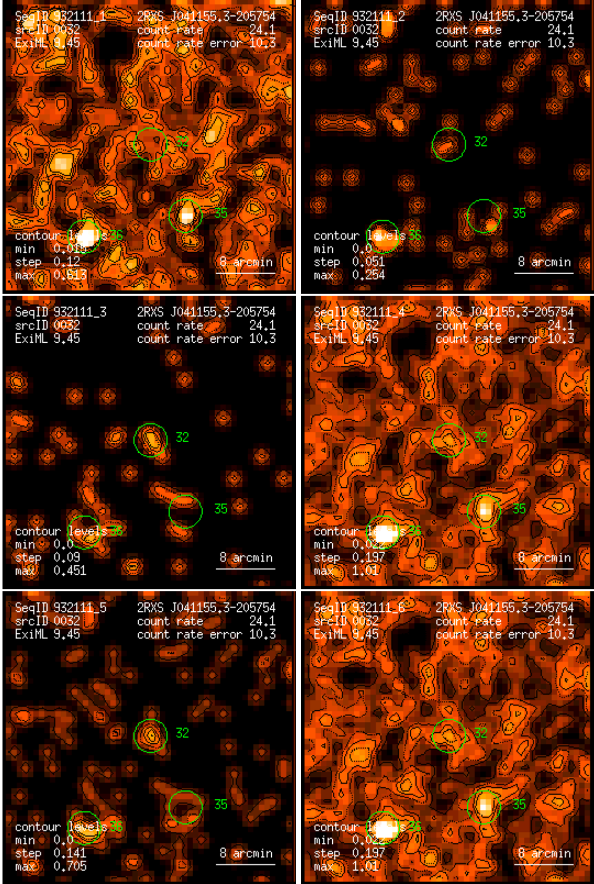
Figure 32: RASS 932111: detection 0032: band rate images, Gaussian filter: (1) PSPC channels 11 – 41, (2) 52 – 90, (3) 91 – 201, (4) 11 – 235, (5) 52 – 201, (6) 11 – 201. Broad band rates in counts/ks. Band rate contour levels in counts/ks/arcmin 2 .
