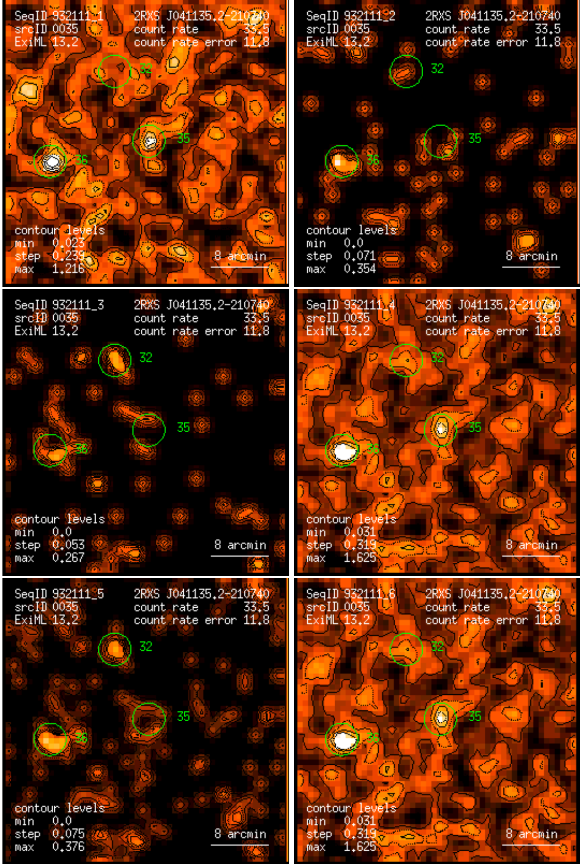
Figure 35: RASS 932111: detection 0035: band rate images, Gaussian filter: (1) PSPC channels 11 – 41, (2) 52 – 90, (3) 91 – 201, (4) 11 – 235, (5) 52 – 201, (6) 11 – 201. Broad band rates in counts/ks. Band rate contour levels in counts/ks/arcmin 2 .
