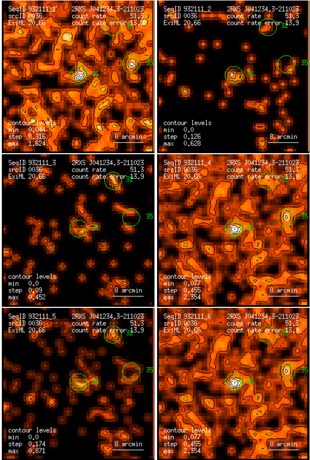
Figure 36: RASS 932111: detection 0036: band rate images, Gaussian filter: (1) PSPC channels 11 – 41, (2) 52 – 90, (3) 91 – 201, (4) 11 – 235, (5) 52 – 201, (6) 11 – 201. Broad band rates in counts/ks. Band rate contour levels in counts/ks/arcmin 2 .
