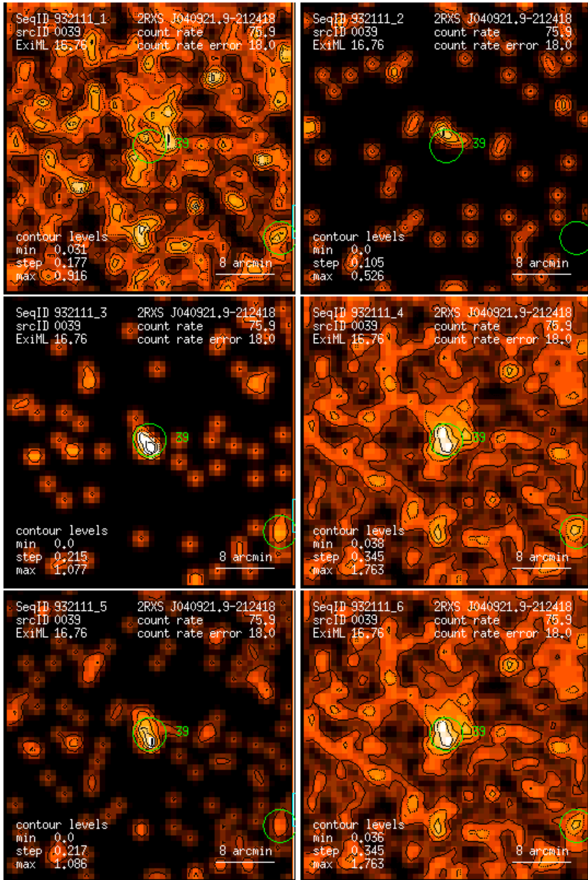
Figure 39: RASS 932111: detection 0039: band rate images, Gaussian filter: (1) PSPC channels 11 – 41, (2) 52 – 90, (3) 91 – 201, (4) 11 – 235, (5) 52 – 201, (6) 11 – 201. Broad band rates in counts/ks. Band rate contour levels in counts/ks/arcmin 2 .
