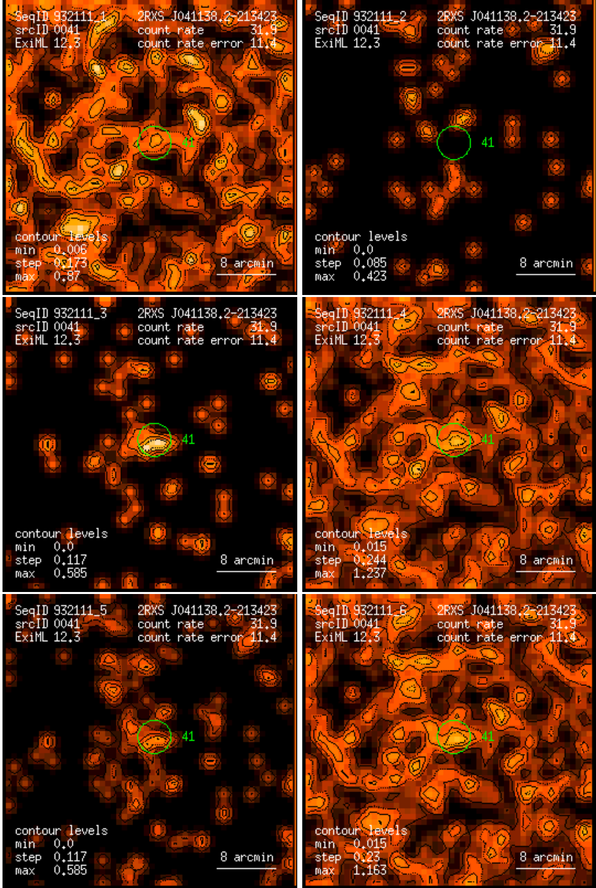
Figure 41: RASS 932111: detection 0041: band rate images, Gaussian filter: (1) PSPC channels 11 – 41, (2) 52 – 90, (3) 91 – 201, (4) 11 – 235, (5) 52 – 201, (6) 11 – 201. Broad band rates in counts/ks. Band rate contour levels in counts/ks/arcmin 2 .
