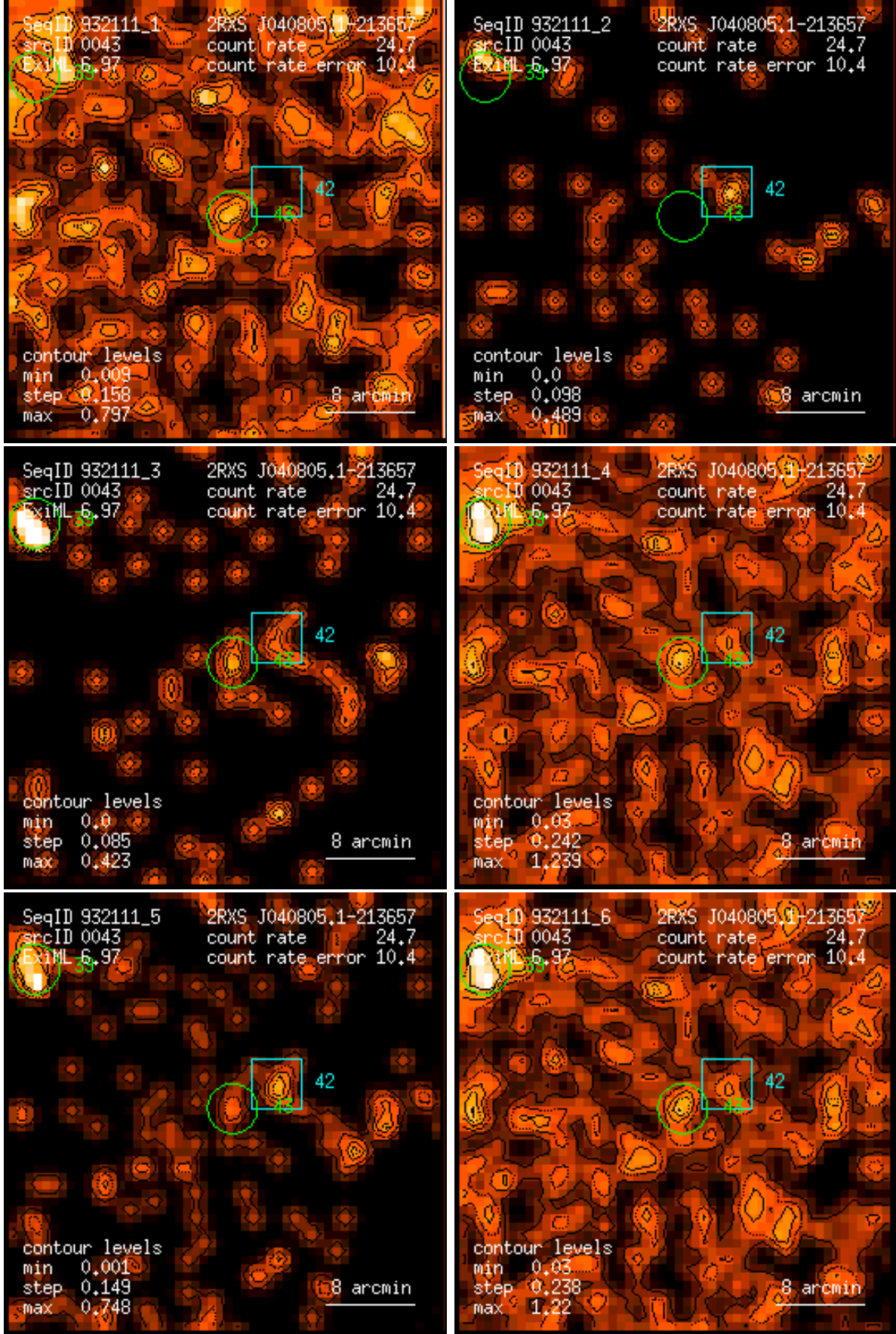
Figure 43: RASS 932111: detection 0043: band rate images, Gaussian filter: (1) PSPC channels 11 – 41, (2) 52 – 90, (3) 91 – 201, (4) 11 – 235, (5) 52 – 201, (6) 11 – 201. Broad band rates in counts/ks. Band rate contour levels in counts/ks/arcmin 2 .
