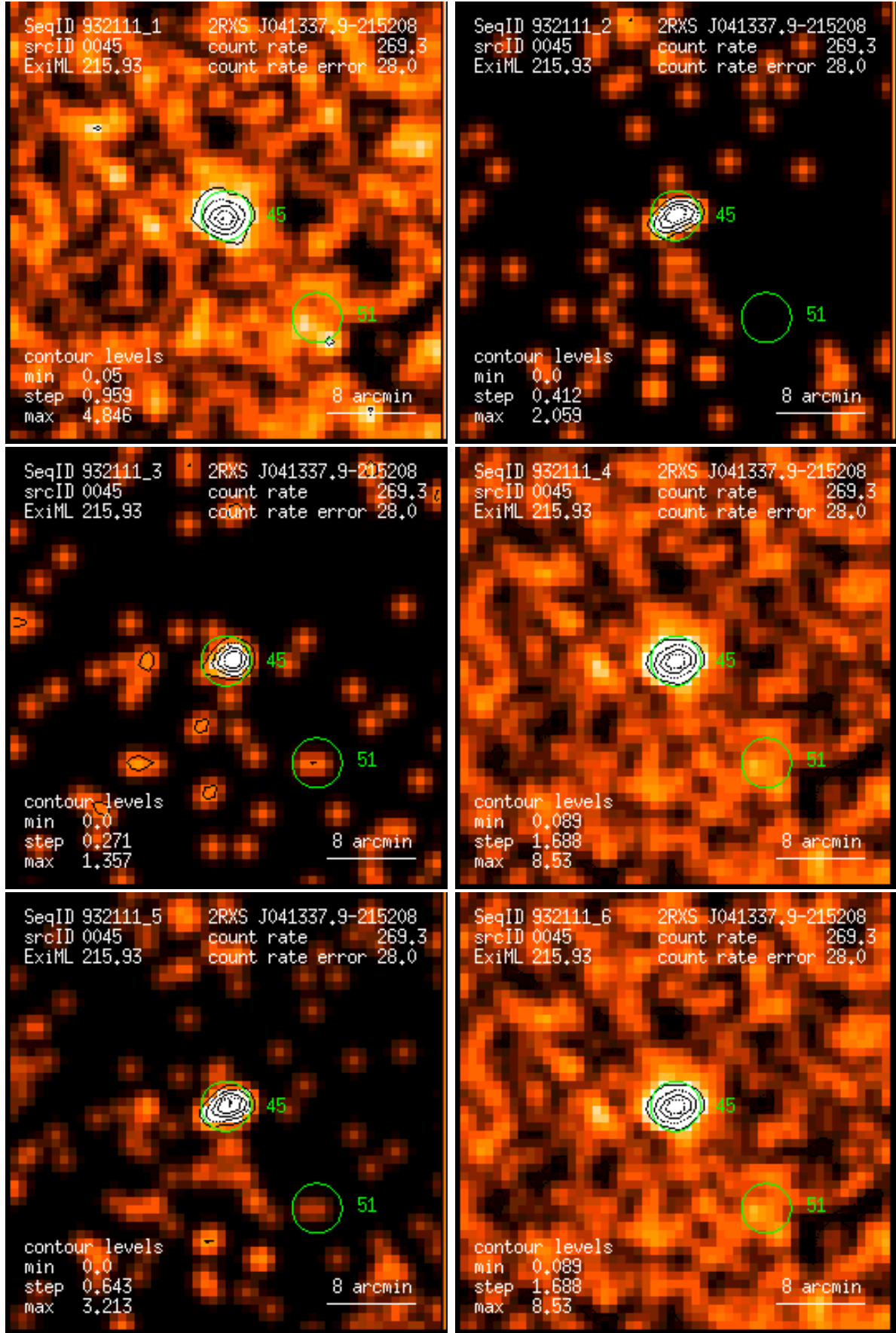
Figure 45: RASS 932111: detection 0045: band rate images, Gaussian filter: (1) PSPC channels 11 – 41, (2) 52 – 90, (3) 91 – 201, (4) 11 – 235, (5) 52 – 201, (6) 11 – 201. Broad band rates in counts/ks. Band rate contour levels in counts/ks/arcmin 2 .
