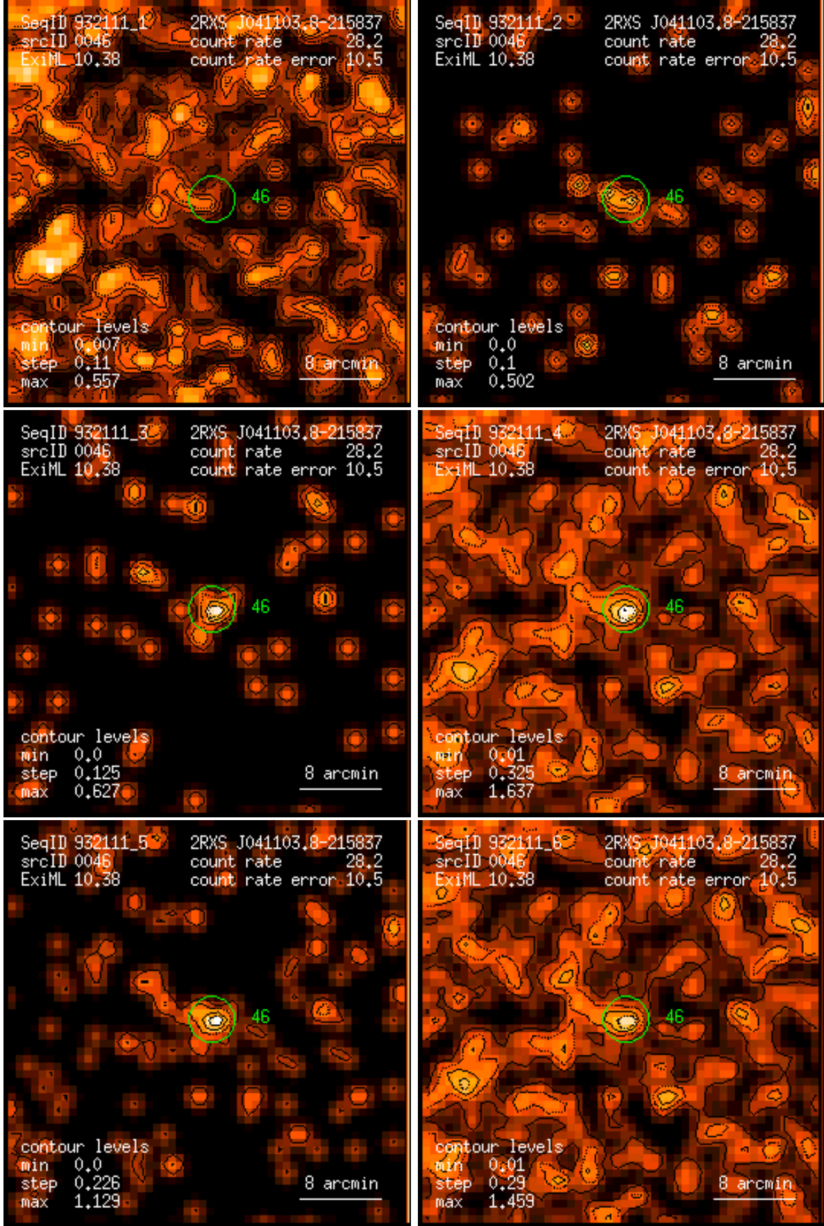
Figure 46: RASS 932111: detection 0046: band rate images, Gaussian filter: (1) PSPC channels 11 – 41, (2) 52 – 90, (3) 91 – 201, (4) 11 – 235, (5) 52 – 201, (6) 11 – 201. Broad band rates in counts/ks. Band rate contour levels in counts/ks/arcmin 2 .
