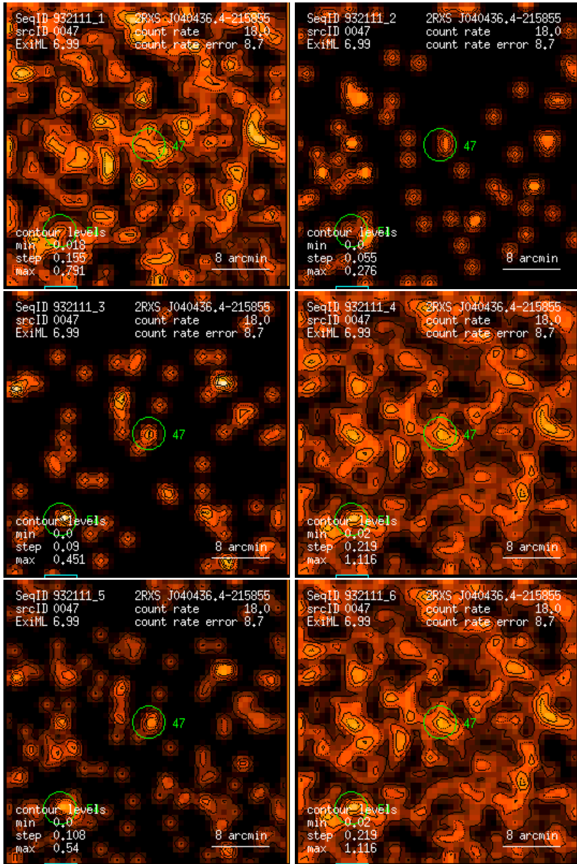
Figure 47: RASS 932111: detection 0047: band rate images, Gaussian filter: (1) PSPC channels 11 – 41, (2) 52 – 90, (3) 91 – 201, (4) 11 – 235, (5) 52 – 201, (6) 11 – 201. Broad band rates in counts/ks. Band rate contour levels in counts/ks/arcmin 2 .
