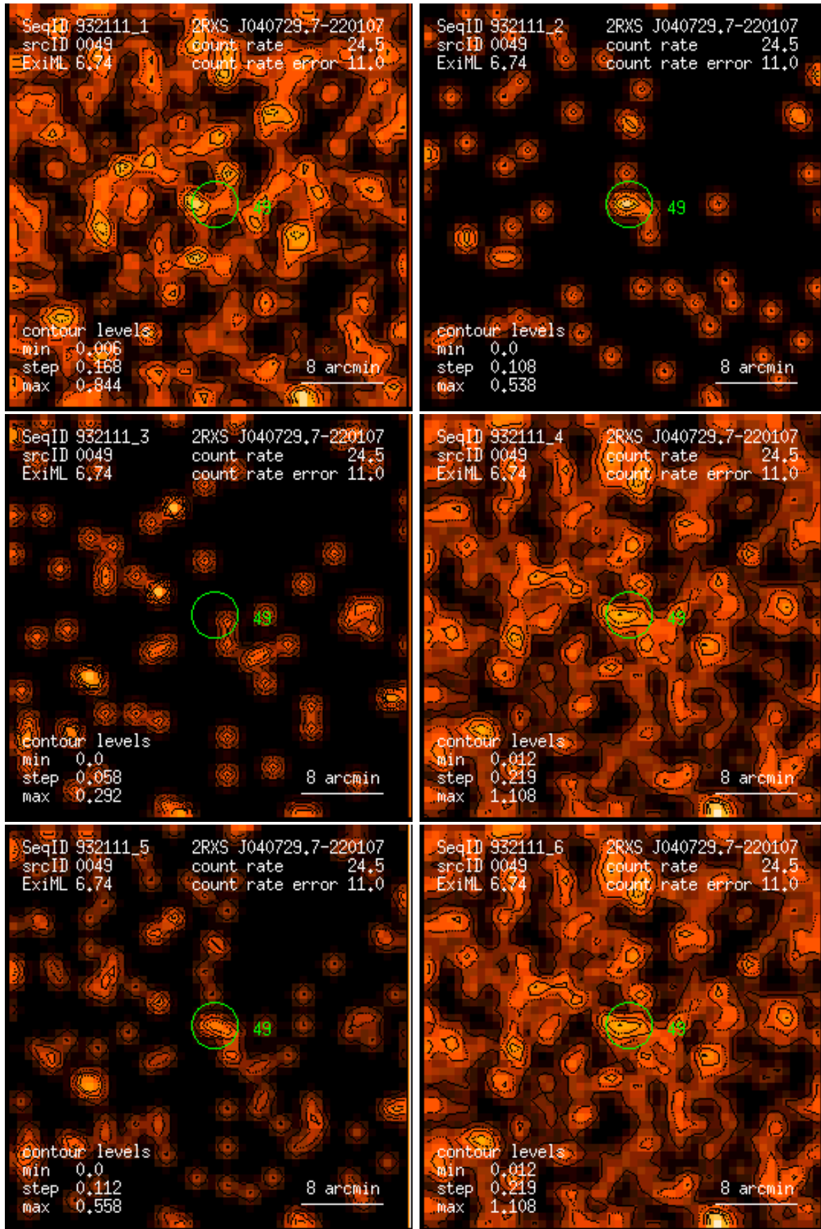
Figure 49: RASS 932111: detection 0049: band rate images, Gaussian filter: (1) PSPC channels 11 – 41, (2) 52 – 90, (3) 91 – 201, (4) 11 – 235, (5) 52 – 201, (6) 11 – 201. Broad band rates in counts/ks. Band rate contour levels in counts/ks/arcmin 2 .
