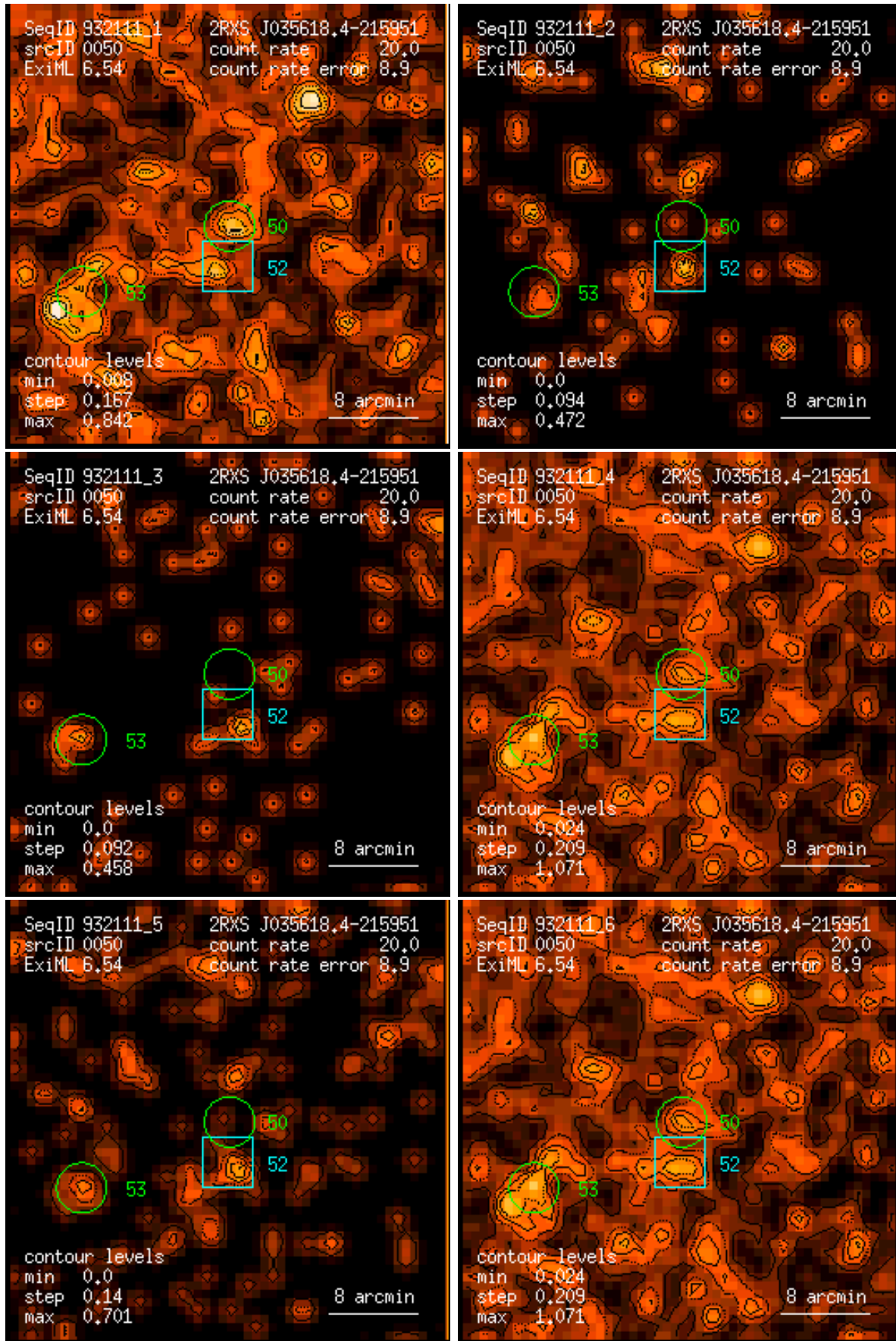
Figure 50: RASS 932111: detection 0050: band rate images, Gaussian filter: (1) PSPC channels 11 – 41, (2) 52 – 90, (3) 91 – 201, (4) 11 – 235, (5) 52 – 201, (6) 11 – 201. Broad band rates in counts/ks. Band rate contour levels in counts/ks/arcmin 2 .
