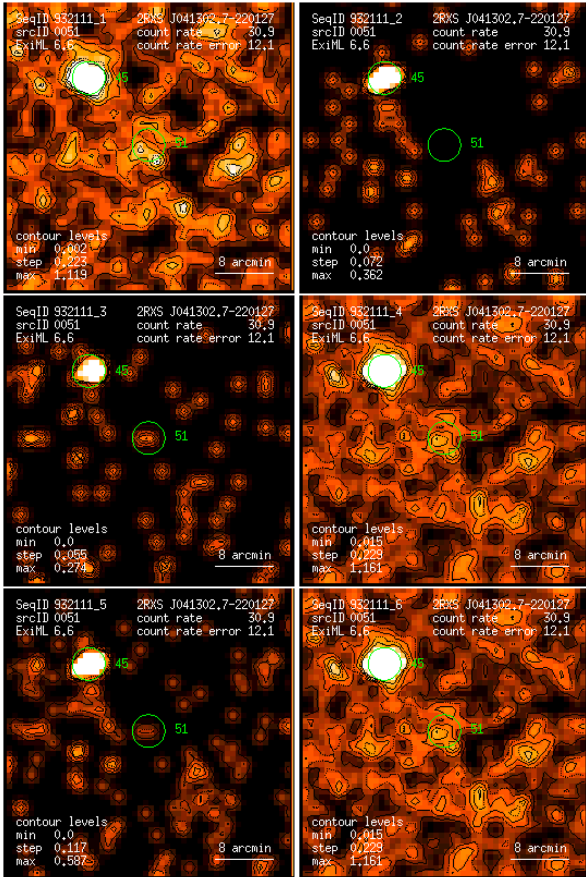
Figure 51: RASS 932111: detection 0051: band rate images, Gaussian filter: (1) PSPC channels 11 – 41, (2) 52 – 90, (3) 91 – 201, (4) 11 – 235, (5) 52 – 201, (6) 11 – 201. Broad band rates in counts/ks. Band rate contour levels in counts/ks/arcmin 2 .
