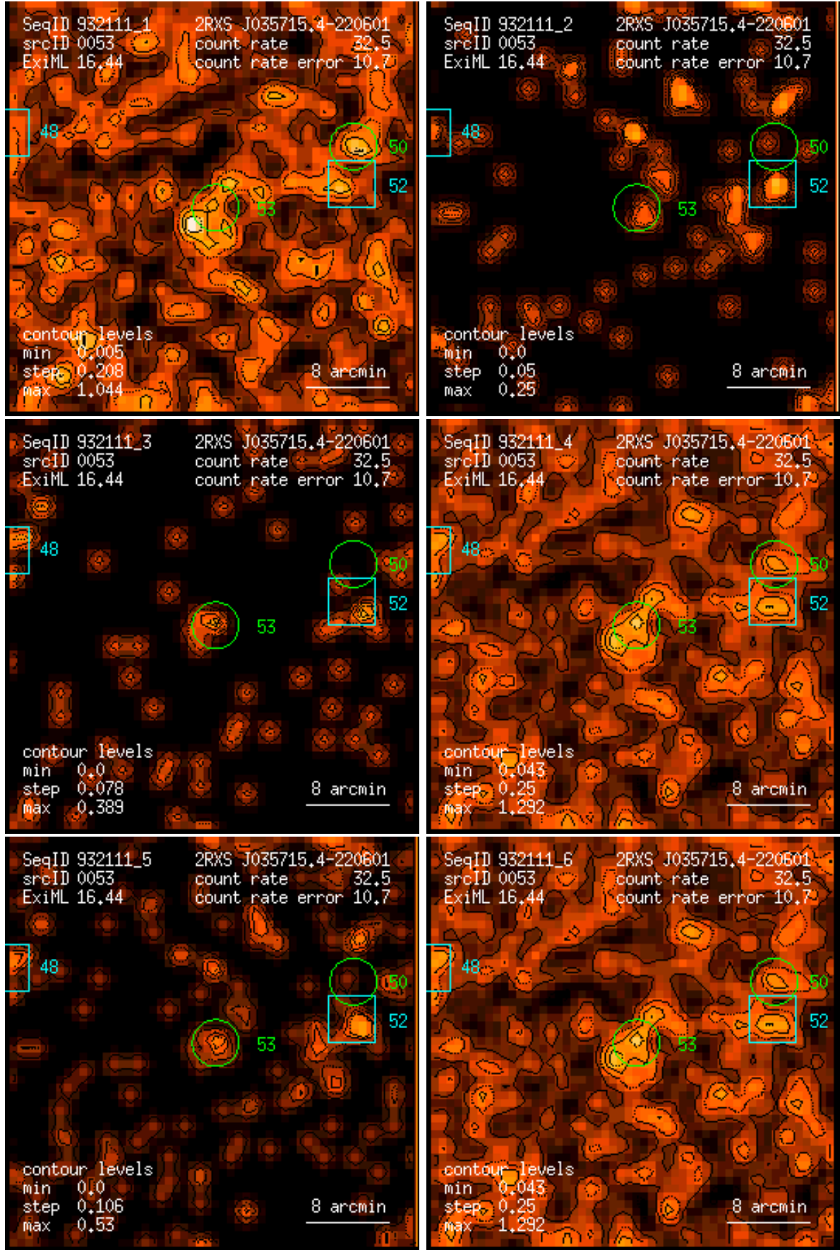
Figure 53: RASS 932111: detection 0053: band rate images, Gaussian filter: (1) PSPC channels 11 – 41, (2) 52 – 90, (3) 91 – 201, (4) 11 – 235, (5) 52 – 201, (6) 11 – 201. Broad band rates in counts/ks. Band rate contour levels in counts/ks/arcmin 2 .
