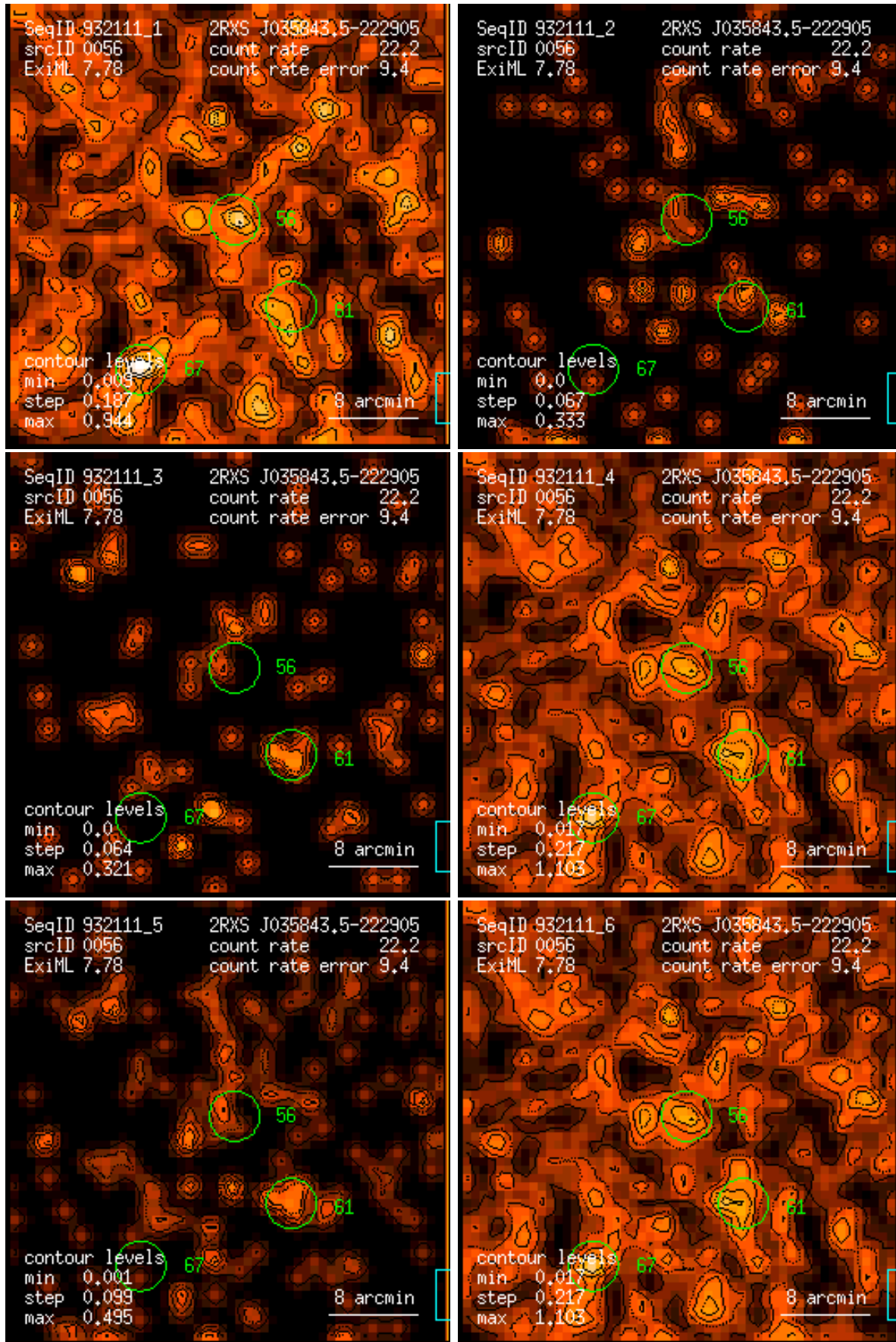
Figure 56: RASS 932111: detection 0056: band rate images, Gaussian filter: (1) PSPC channels 11 – 41, (2) 52 – 90, (3) 91 – 201, (4) 11 – 235, (5) 52 – 201, (6) 11 – 201. Broad band rates in counts/ks. Band rate contour levels in counts/ks/arcmin 2 .
