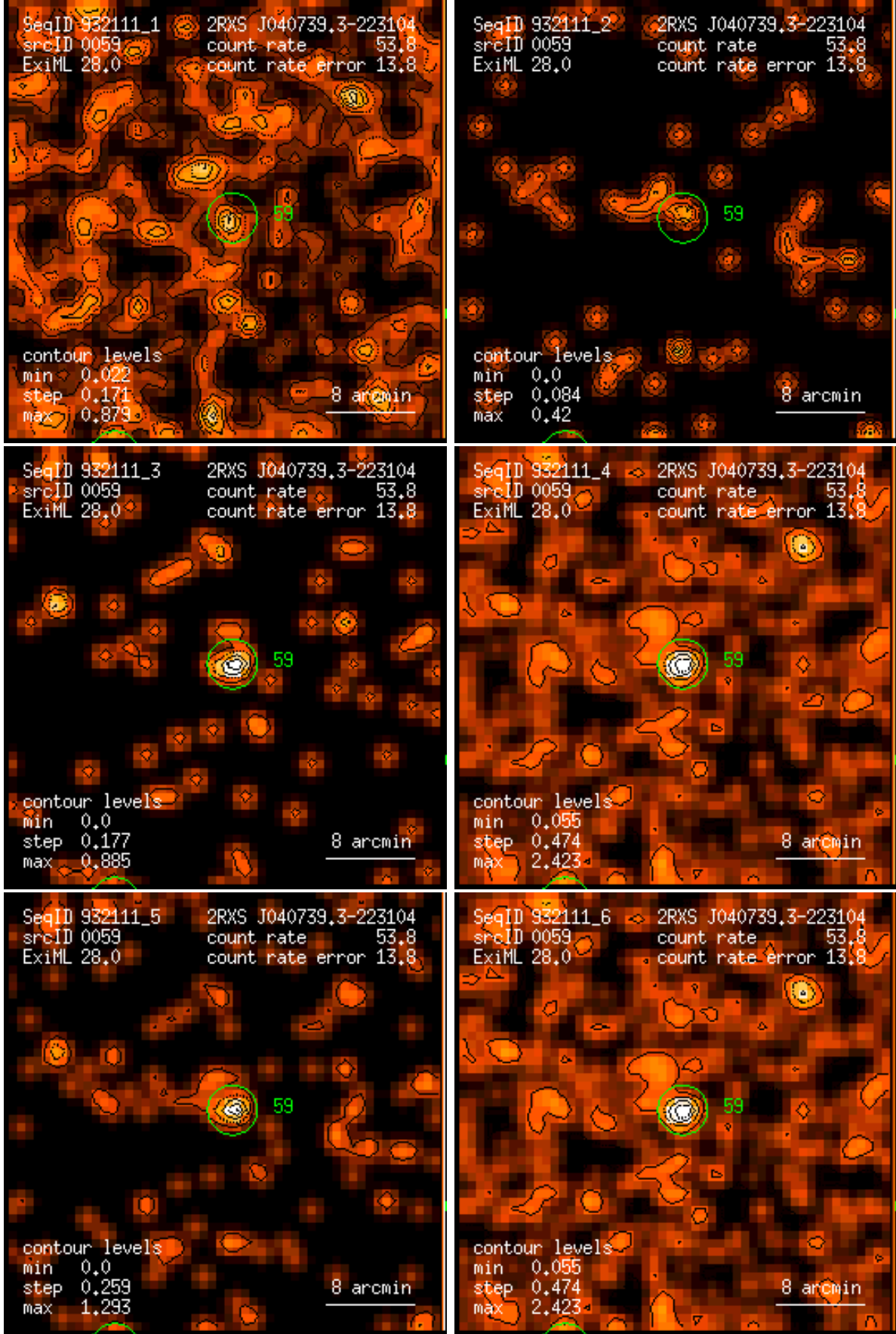
Figure 59: RASS 932111: detection 0059: band rate images, Gaussian filter: (1) PSPC channels 11 – 41, (2) 52 – 90, (3) 91 – 201, (4) 11 – 235, (5) 52 – 201, (6) 11 – 201. Broad band rates in counts/ks. Band rate contour levels in counts/ks/arcmin 2 .
