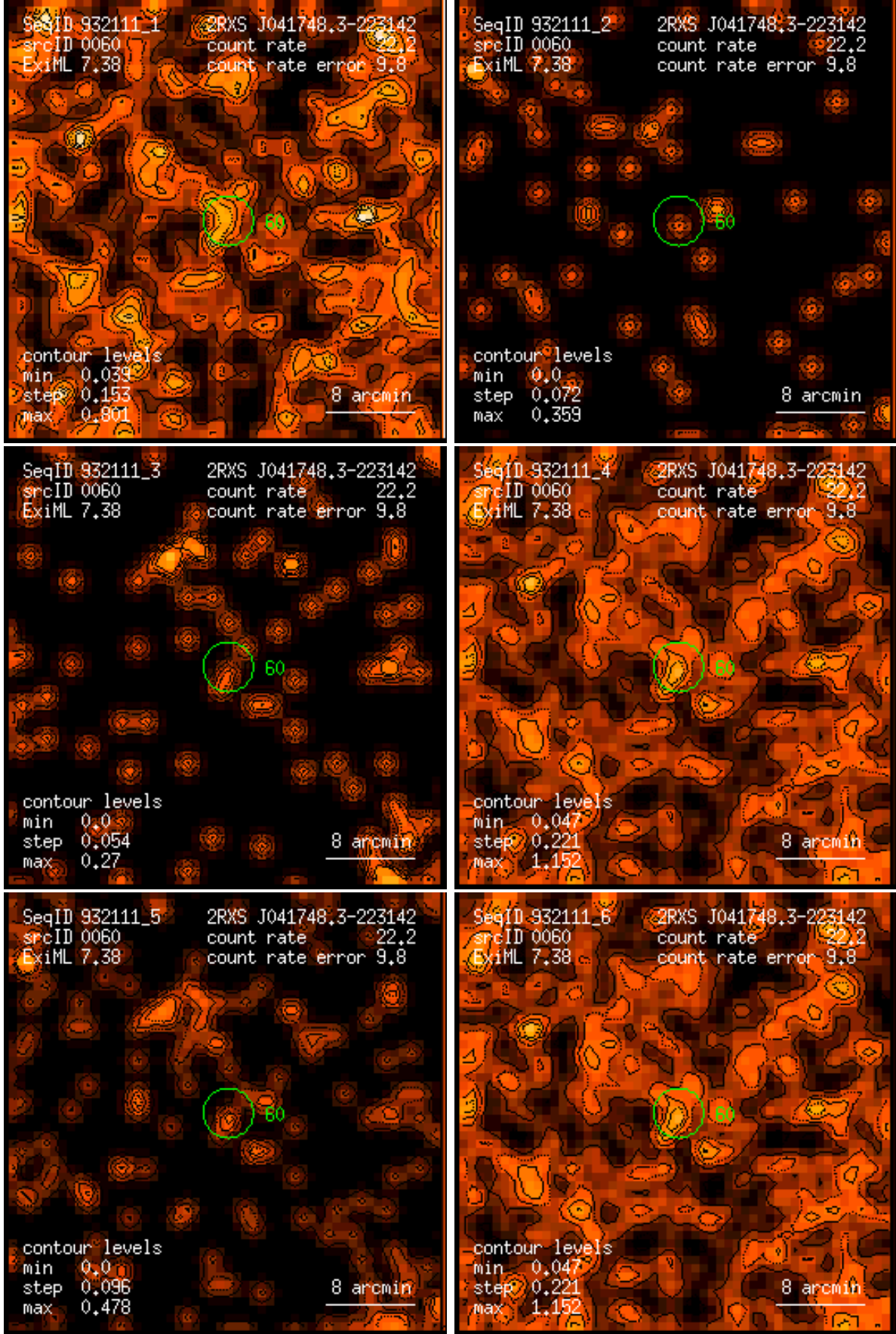
Figure 60: RASS 932111: detection 0060: band rate images, Gaussian filter: (1) PSPC channels 11 – 41, (2) 52 – 90, (3) 91 – 201, (4) 11 – 235, (5) 52 – 201, (6) 11 – 201. Broad band rates in counts/ks. Band rate contour levels in counts/ks/arcmin 2 .
