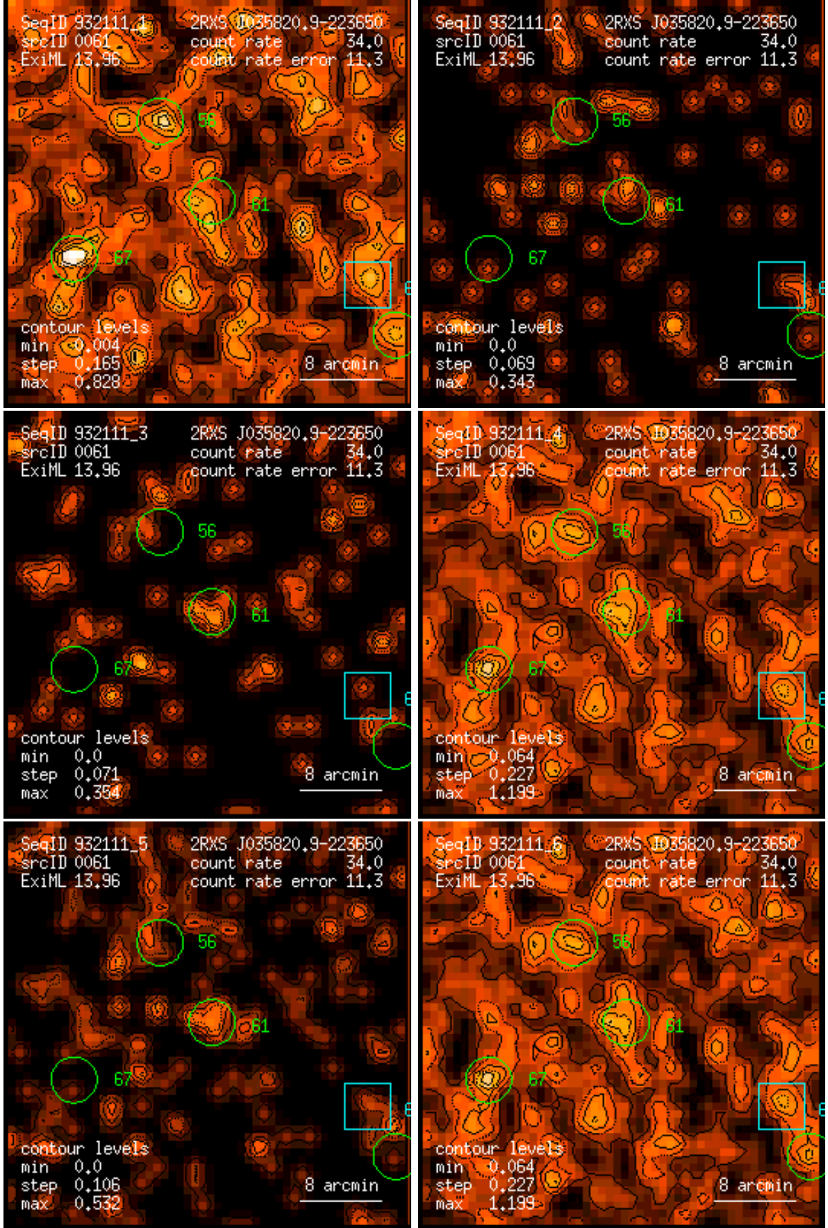
Figure 61: RASS 932111: detection 0061: band rate images, Gaussian filter: (1) PSPC channels 11 – 41, (2) 52 – 90, (3) 91 – 201, (4) 11 – 235, (5) 52 – 201, (6) 11 – 201. Broad band rates in counts/ks. Band rate contour levels in counts/ks/arcmin 2 .
