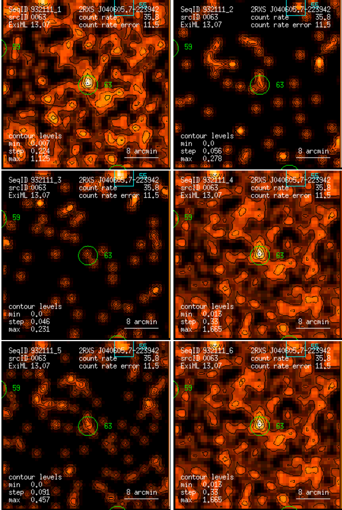
Figure 63: RASS 932111: detection 0063: band rate images, Gaussian filter: (1) PSPC channels 11 – 41, (2) 52 – 90, (3) 91 – 201, (4) 11 – 235, (5) 52 – 201, (6) 11 – 201. Broad band rates in counts/ks. Band rate contour levels in counts/ks/arcmin 2 .
