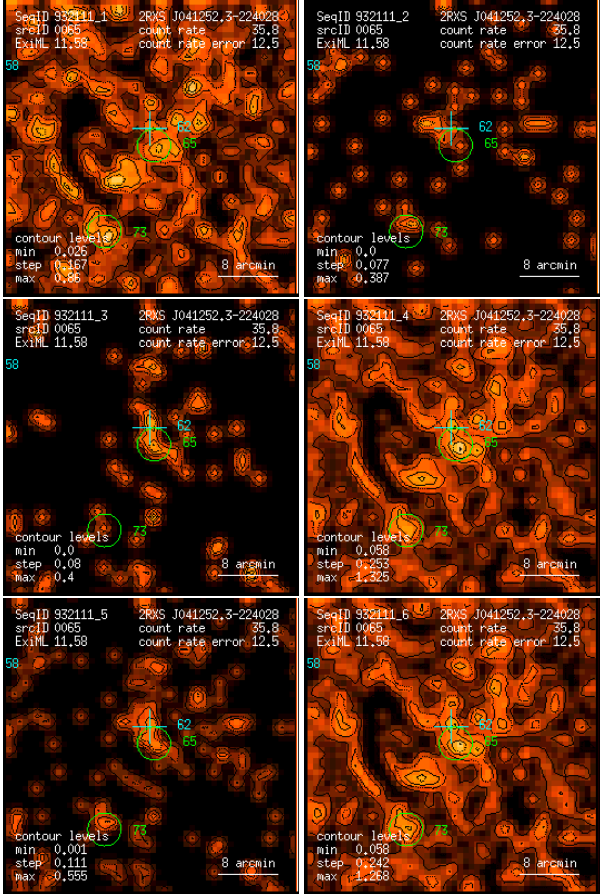
Figure 65: RASS 932111: detection 0065: band rate images, Gaussian filter: (1) PSPC channels 11 – 41, (2) 52 – 90, (3) 91 – 201, (4) 11 – 235, (5) 52 – 201, (6) 11 – 201. Broad band rates in counts/ks. Band rate contour levels in counts/ks/arcmin 2 .
