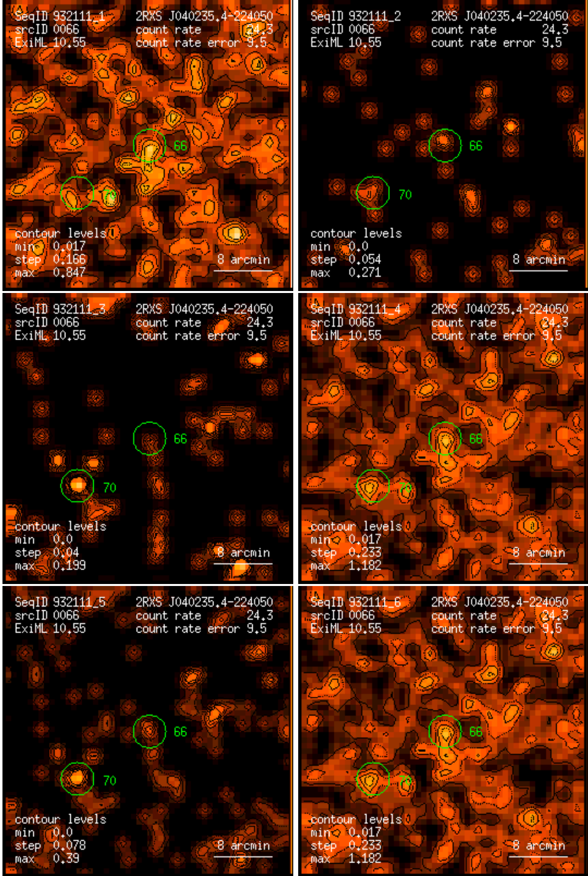
Figure 66: RASS 932111: detection 0066: band rate images, Gaussian filter: (1) PSPC channels 11 – 41, (2) 52 – 90, (3) 91 – 201, (4) 11 – 235, (5) 52 – 201, (6) 11 – 201. Broad band rates in counts/ks. Band rate contour levels in counts/ks/arcmin 2 .
